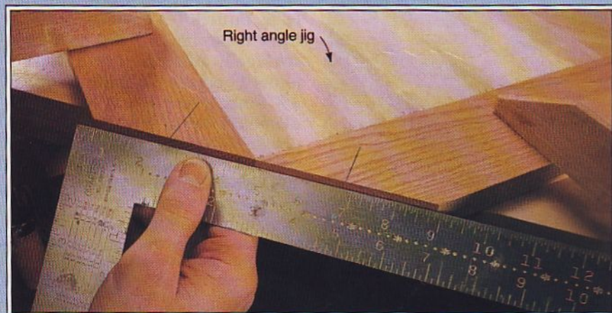
A straightedge and scrap of wood or plywood cut at 90° help you align and clamp the ends of workpieces mitered at 45°.
