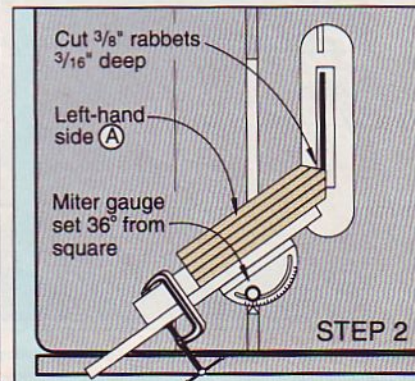
Using a miter gauge and a dado blade mounted to your tablesaw, cut a rabbet along the bottom front edge of each tray side piece.
