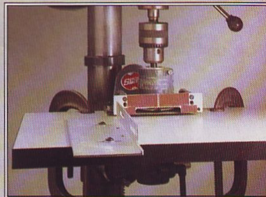
Shopsmith 555485 mounted to a drill press (C-clamps not included)
