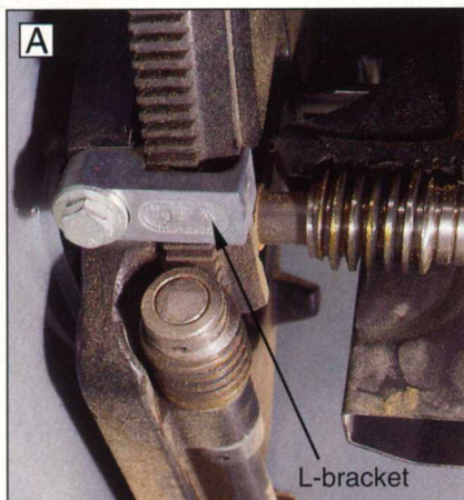
An L-bracket on the Delta prevents its yoke-style trunnion carriage from twisting when adjusted for 45° bevel cuts.
