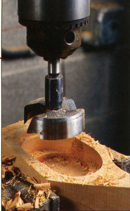
After sawing a ladle to shape, the bowl is roughly bored out at the drill press with overlapping bites of a Forstner bit.
