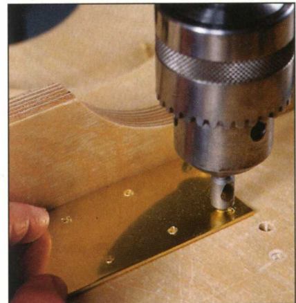
Make a slight depression on the inside face of the brass plates with a countersink bit to remove the ridge.
