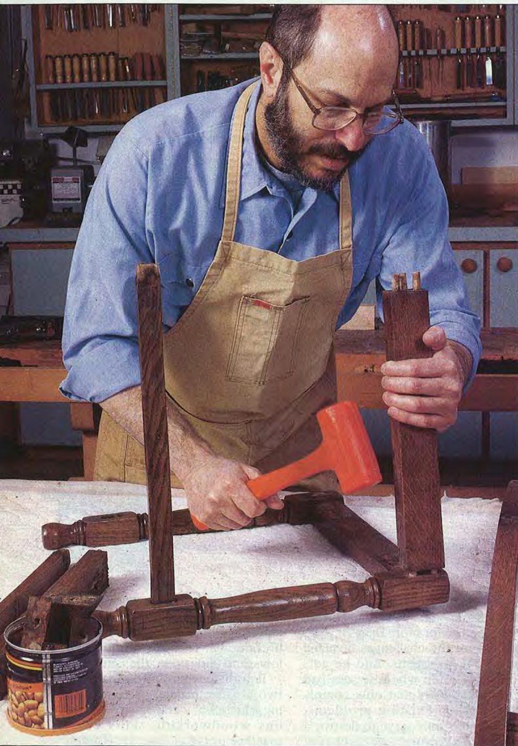
To protect the wood when knocking an old chair's joints loose, Bob Flexner relies on a dead-blow hammer and a cushioned tabletop. Solid hits make the job go quickly.
