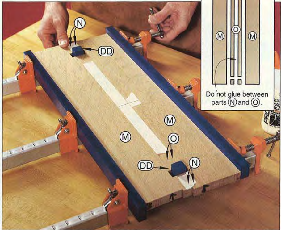
The top's outer edges and mortises are overlength, so ends need not look perfect. After joining these assemblies to the center, you will trim the top to finished length.
