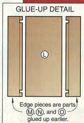
The top's outer edges and mortises are overlength, so ends need not look perfect. After joining these assemblies to the center, you will trim the top to finished length.
