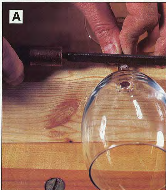
A Score the glass stem all around with a file. Support the stem with a scrapwood block.
