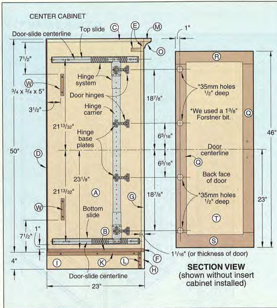
C Locate the top slide's position in the cabinet, drill the mounting holes, and screw the slide in place.
