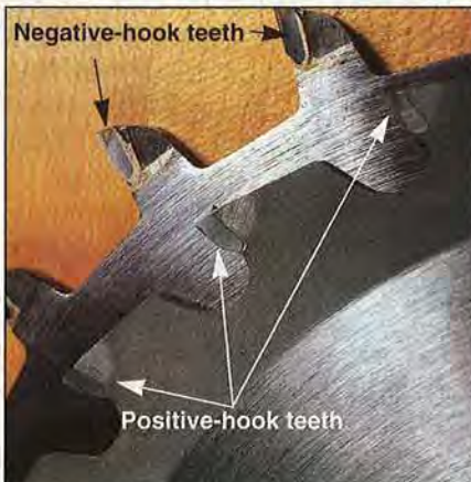
Negative-hook teeth cut more cleanly than positive-hook teeth that cut with greater ease and speed.
