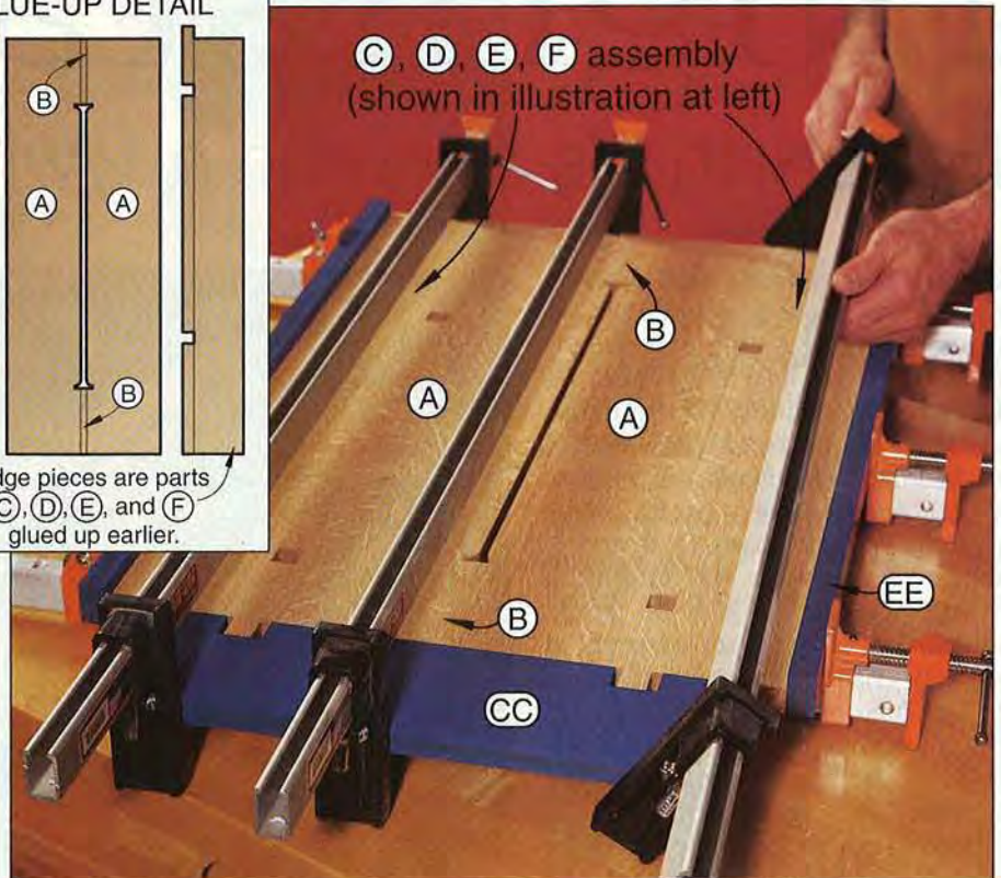
Fixture CC ensures a straight top when gluing up the side panel. Keep surfaces flush when gluing up all parts.
