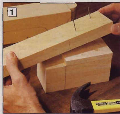
TIP: Drive nails (we used 4d finish nails) into what will be waste areas to prevent laminations from creeping when you clamp them.
