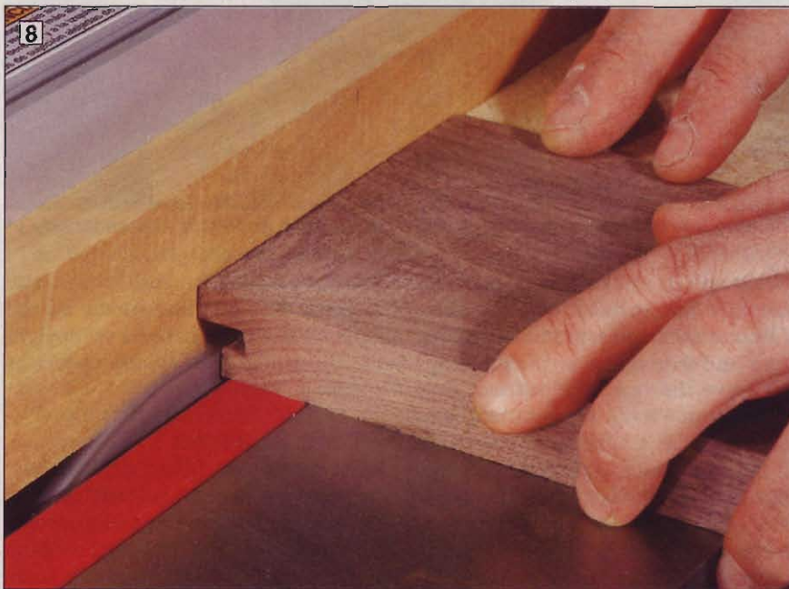
8 After cutting a centered groove in the end of the drawer front, trim half of the rear tongue to make a locking joint.
