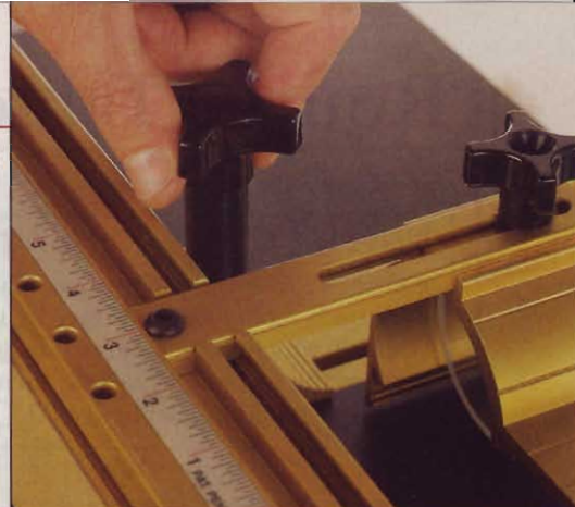
A paragon of comfort and accessibility, the large knobs on the JessEm Rout-R-Slide extend above the fence.
