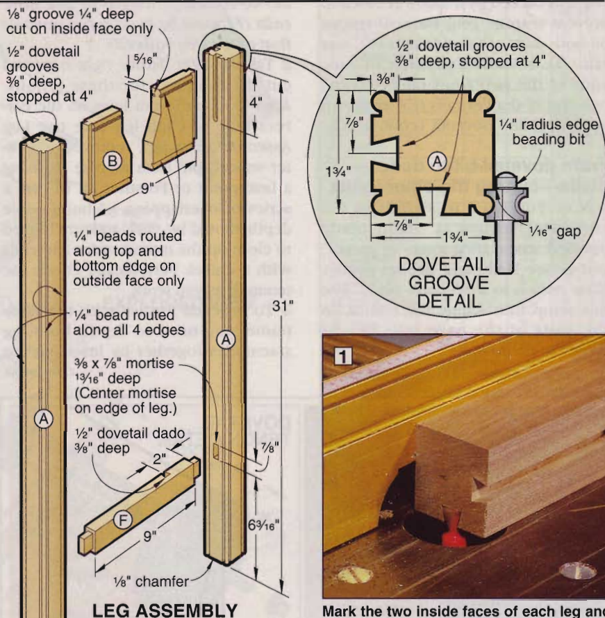
LEG ASSEMBLY
