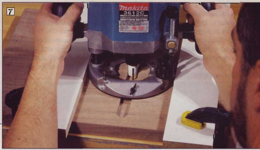
Clamp guide boards in place to rout drawer stopped dados in the underside of the tabletop.
