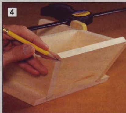
4 The front panel (L), temporarily placed in the center of the box, helps hold the box sides in position while you fit the back panel and mark its width (height).
