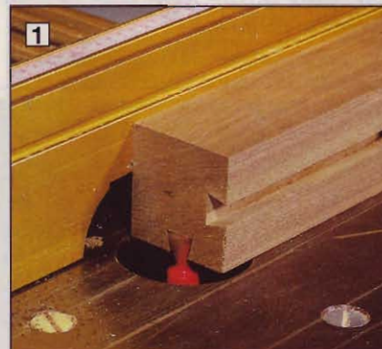
1 Mark the two inside faces of each leg and rout 4"-long dovetail slots at the top. A stopblock limits the workpiece travel.
