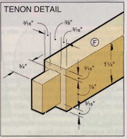
Fit an auxiliary fence to your tablesaw and use a 3/4" dado blade to cut the tenons on the base rails.
