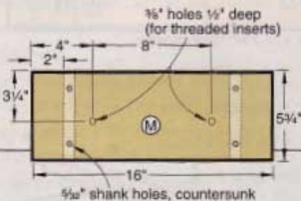
BENCH-MOUNT PARTS VIEW
