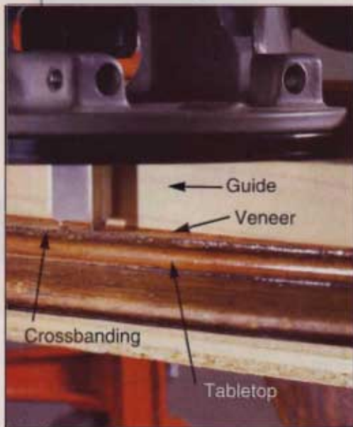
The router bit should just cut through the veneer to the crossbanding or other base material.
