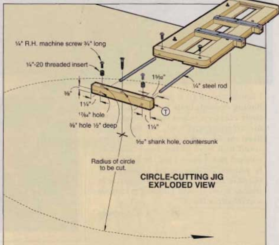
With this special circle-jig attachment, you can rout arcs and circles in large workpieces such as sheet goods.
