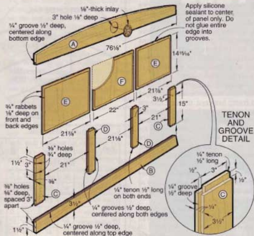
BACK FRAME
