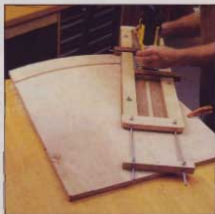
With this special circle-jig attachment, you can rout arcs and circles in large workpieces such as sheet goods.
