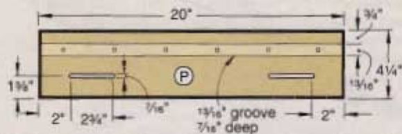
BENCH-MOUNT PARTS VIEW
