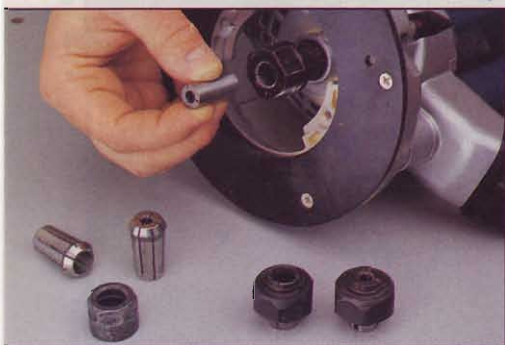
To go from ½" to ¼" bits, some manufacturers provide a reducer that fits into the ½" collet. Others, such as DeWalt (left) and Porter-Cable (right) use separate ¼" and ½" collets.
