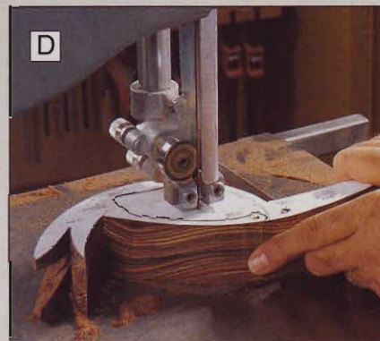
D A 1/8" bandsaw blade will help you saw the sharp inside corners in the box.
