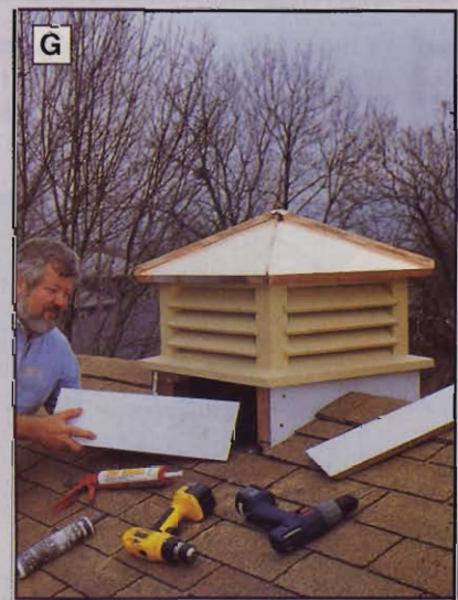
G To prevent moisture from penetrating, the skirting pieces must be cut for a tight fit. Caulk all joints.
