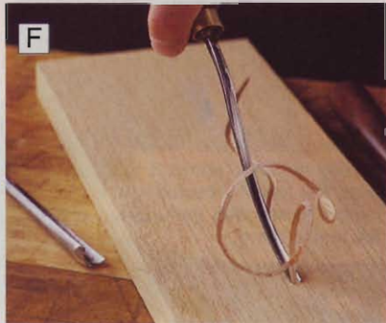
F A sharp tool will leave the sides of the cut and chip smooth. Cuts across the grain give the best indication of a tool's sharpness.
