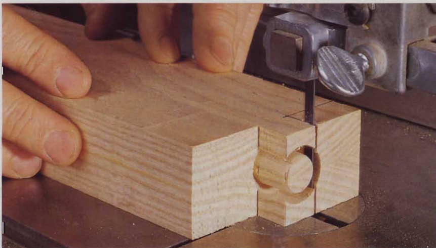
Once you've pinpointed the right location for a tenon, the milling work goes quickly.
