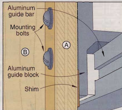
SHIMMING THE TABLE UPRIGHT
