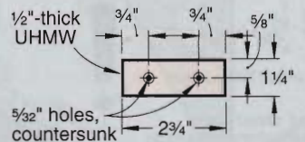
UHMW WEAR BLOCK (2 needed)
