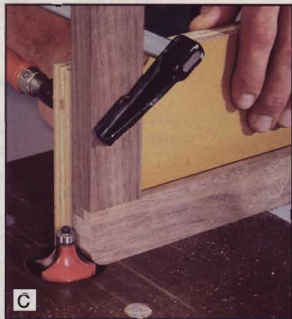
C To prevent tear-out on the trailing faces of the stiles, use an auxiliary fence attached to the miter gauge.
