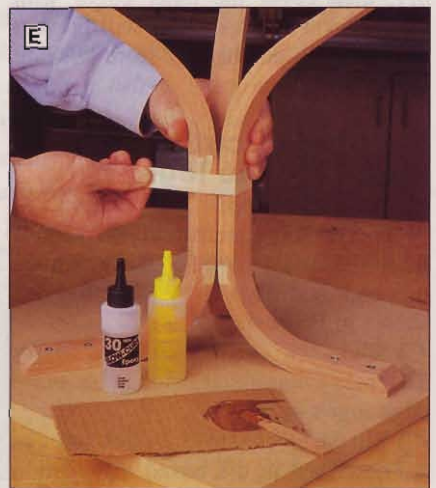
Masking tape holds the legs against the filler block as the epoxy cures. Screws keep the tops of the legs in a flat plane.
