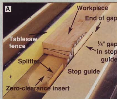
Position the end of the sawn or routed gap in the stop guide with the leading edge of the saw blade.
