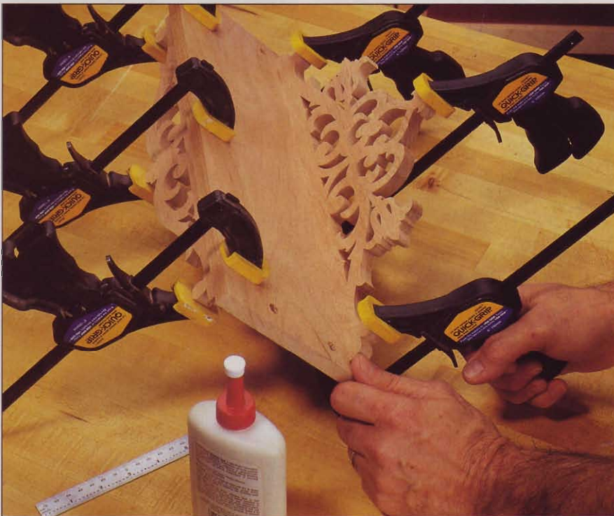
Space the top trim \frac{1}{4} " from the back edge of the top, and position the top apron \frac{1}{2} " from the front edge of the top.
