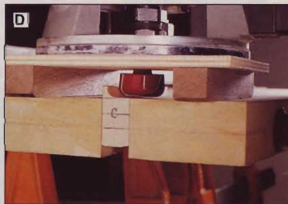
We chamfered the end bottoms of the leg so the other \frac{5}{8} " and \frac{3}{8} " marks align with the other side of the form during the leg tapering.
