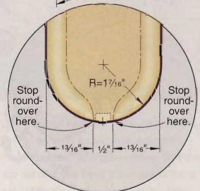
ROUND-OVER DETAIL (TOP VIEW)
