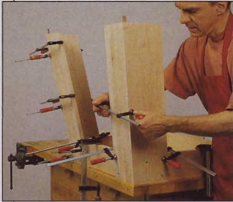
Clamping the legs (D) to the frame (A/B/C) holds them at the proper angle while you finish clamping their length.
