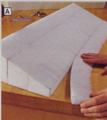
A Arrange the rear pieces for the seat back in a wedge shape, and adhere them with a spray adhesive compatible with foam.
