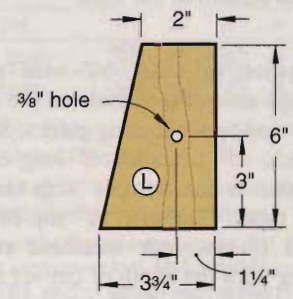
ARM BLOCK
