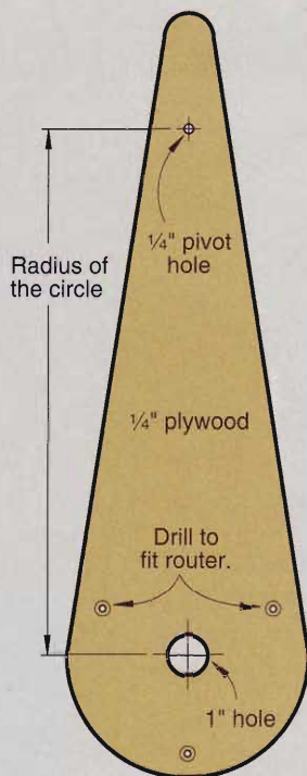
ROUTER TRAMMEL
