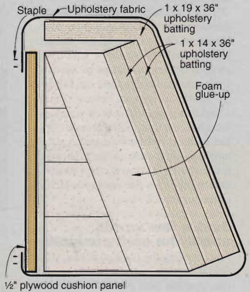
BACK-CUSHION ASSEMBLY
