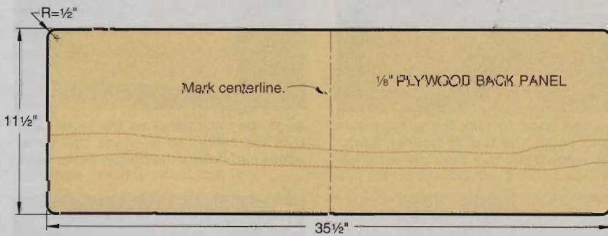
PANEL VIEWS
