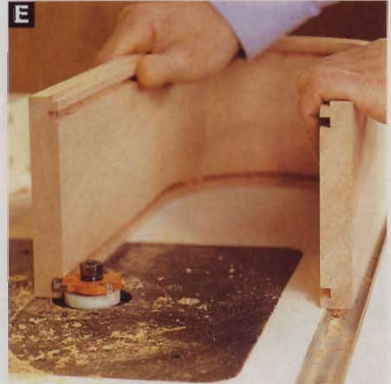
E Rout the grooves with a slot cutter by moving the top/side assembly in a counter-clockwise direction.
