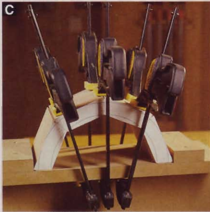
C When clamping the staved top, apply the clamps symmetrically, and use just enough muscle to close the joints.
