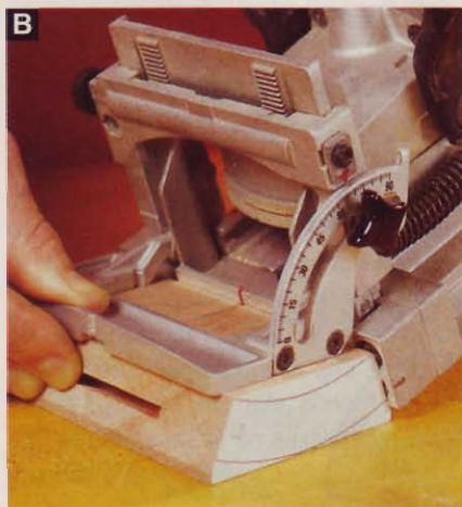
B Center and cut the #20 biscuit slot into the end of each stave.
