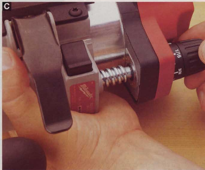
C Tiny changes to cutting depth are easier and more accurate on a router with a threaded-rod depth system.
