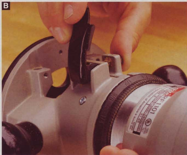
B We found lever locks, such as this one on the Makita RF1101, simple, fast, and secure.
