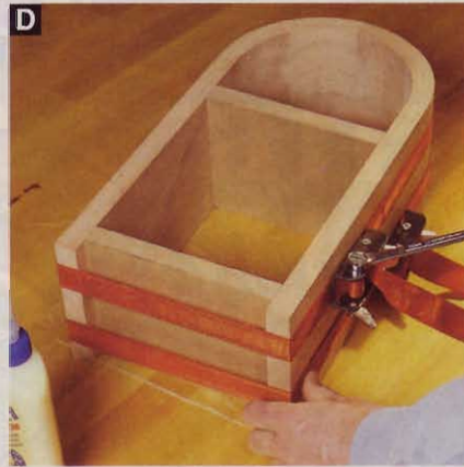
D A pair of band clamps snugs the staved top to the sides while the scrapwood spacers keep the sides parallel.
