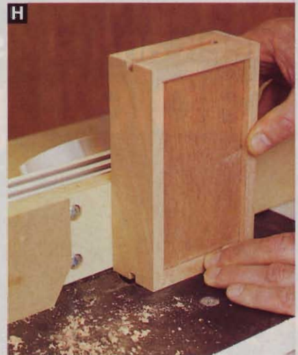
H Carefully centering the bit in the drawer's side, rout grooves into both sides with this one setup.
