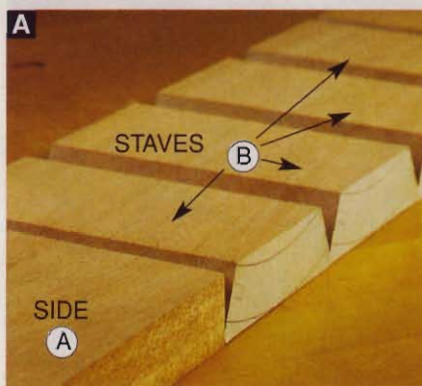
Cutting all of the sides and staves from a single length of lumber will ensure consistent color and continuous grain in the completed clock.
