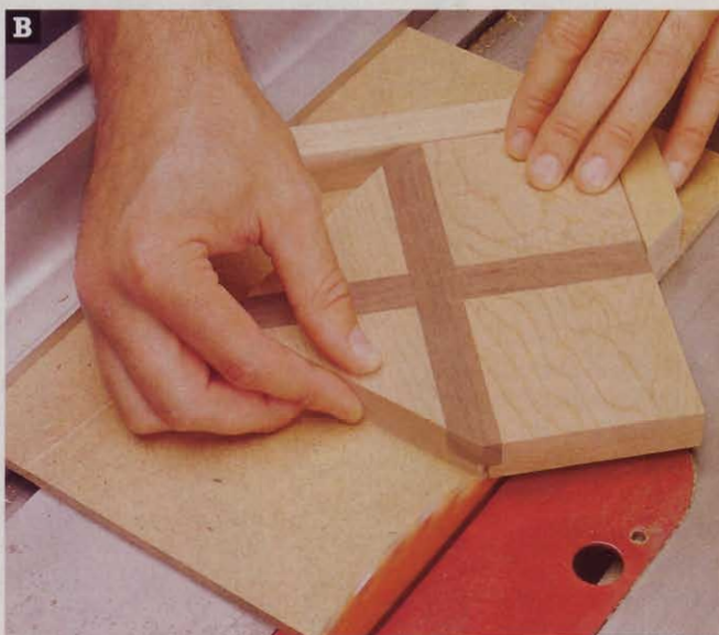
Position the tablesaw fence so the corner-cutting jig just slips past the blade. Hold each blank securely against the jig cleats as you cut four of the blanks down to 4 1/4 x 4 1/4".
