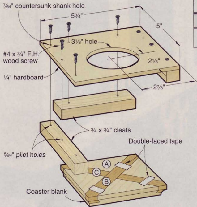
6 RECESS-ROUTING JIG
