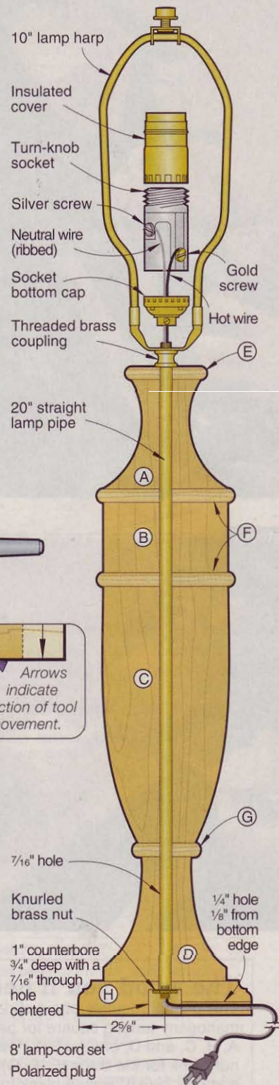
SECTION VIEW
