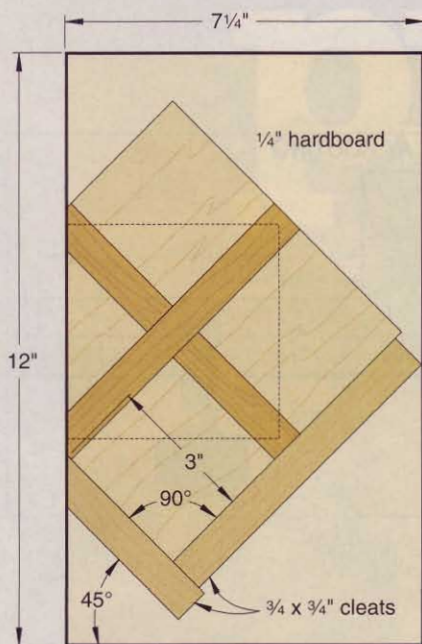
3 CORNER-CUTTING JIG
