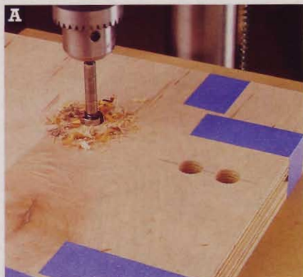
A Use a Forstner bit and your drill press to drill the slot-defining holes in the inside panels (D).
