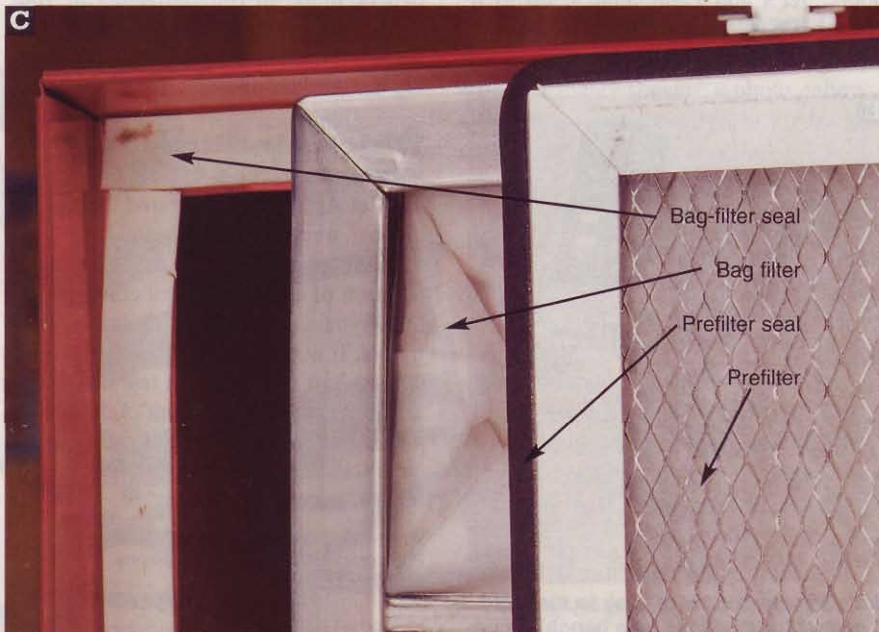
To reduce the amount of dust bypassing the filters, Penn State puts a foam seal around the prefilter and another behind the bag filter.
