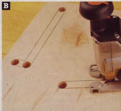
B Use a couple pieces of scrap lumber to raise the inside panels off your workbench while you jigsaw the slots.
