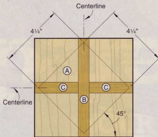
4 COASTER LAYOUT
