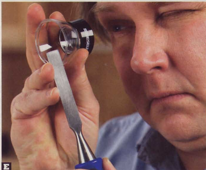
E Most of us need a little magnification to examine the chisel edge for a consistent scratch pattern. This simple loupe allows plenty of light to reach the subject, and magnifies it eight times.
