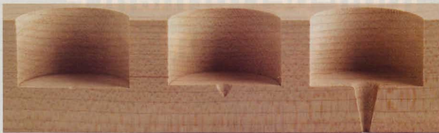
We bored these 1"-deep holes with (from left to right) true Forstner, imported Forstner, and spade bits. Note that the center spur of the spade bit broke through the bottom of the 1 3/4"-thick board.
