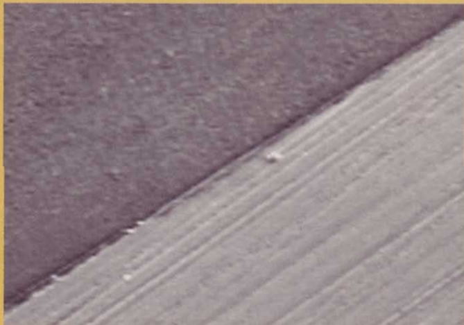
Here's one tiny section of a chisel edge that was sharpened with the side-to-side method. The view is magnified 150 times. At that extreme, you can see slight scratches left even after stropping.
