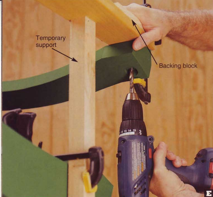
Using the holes in the splat rail assembly (G/H) as guides, drill \frac{3}{8} " holes through the arms. Backing blocks prevent splintering.
