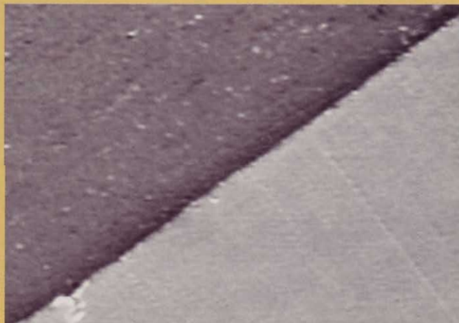
Also magnified 150 times, this chisel was sharpened on a high-end system. The scratches run perpendicular to the edge, and are less prominent than those at left , but there's little difference in sharpness.
