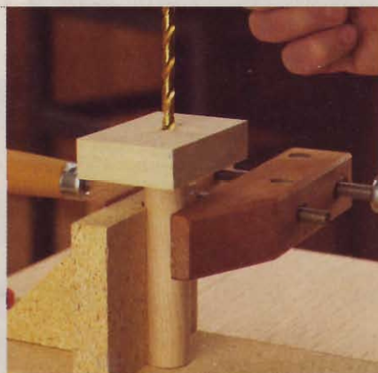
BRAD-POINT BIT
