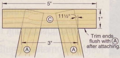
1a TOP RAIL DETAIL
