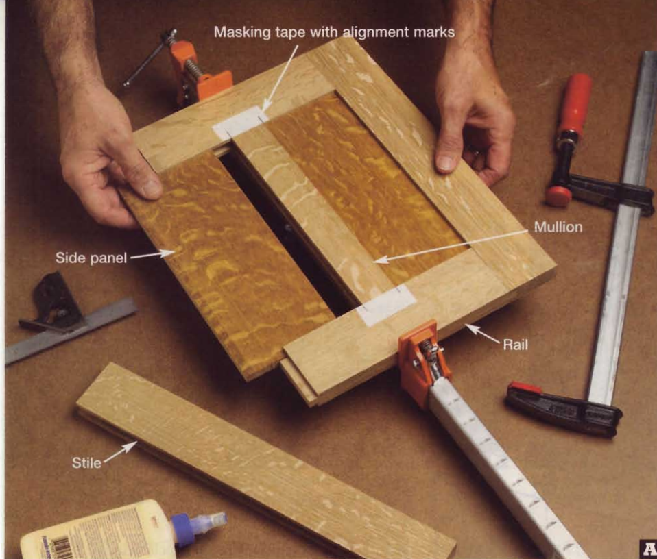
With the mullion and rails assembled, slide in the panels without glue. Glue and clamp the stiles to the rails, keeping them flush at the top and bottom.
