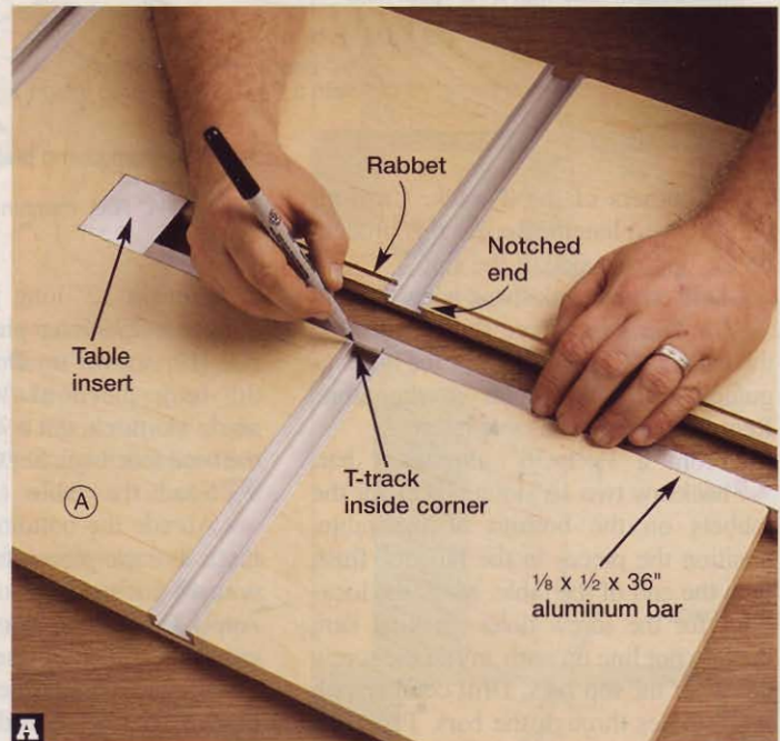
Using a fine-tip permanent marker, mark the bar exactly at the inside corners of the T-track and at the table's end and crosscut to length.
