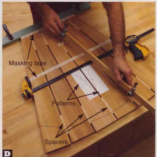
D Inserting \frac{3}{8} " spacers, position the other splats. Adhere the tree patterns with spray adhesive. Apply masking tape, and mark the hole locations. Draw the radius.
