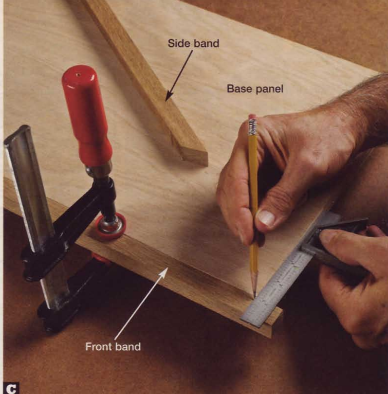
...then using a sharp pencil and a ruler, mark the miter's heel on the front band at the panel's second corner.
