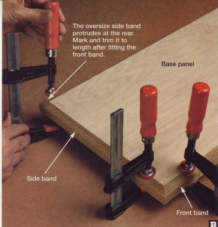
Fit the mitered ends of the side and front bands around the panel's first corner, temporarily clamping them in place...
