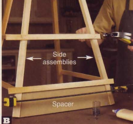
B Clamp the spacer between the assemblies' legs at one end. Attach the rail blanks, aligning them with the adjoining rails.
