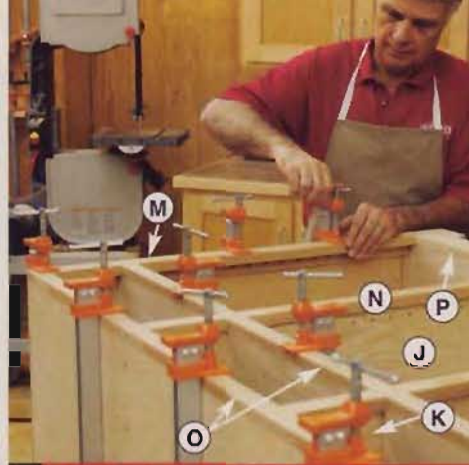
E ATTACH THE FACE FRAME Clamp the face frame (M/N/O/P) to the case around the perimeter and on the inside to ensure it's securely attached to the lower and upper dividers (J, K).
