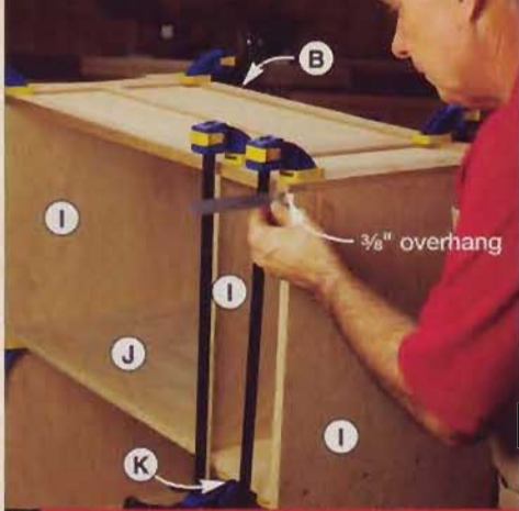
C GLUE THE SIDE TO THE CASE Position the side assembly so that it overhangs the case's front edge by \frac{3}{8} " while the rabbeted edge of the rear stile (B) is flush with the case's back edge.
