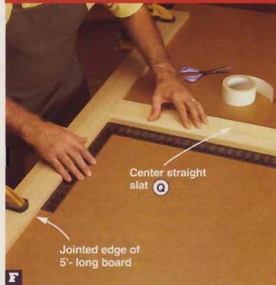
Apply double-faced tape to the back of a straight slat (Q). Center it on the jointed edge of a 5'-long board, align it with a framing square, and stick it to your workbench.
