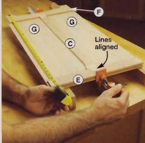
A GLUE THE RAILS AND CENTER STILE
