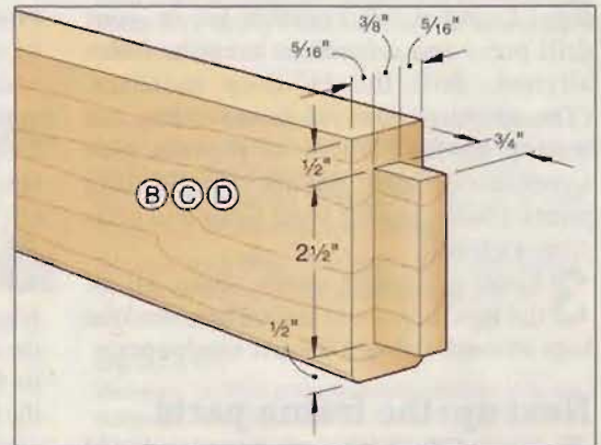
2a TENON DETAIL
