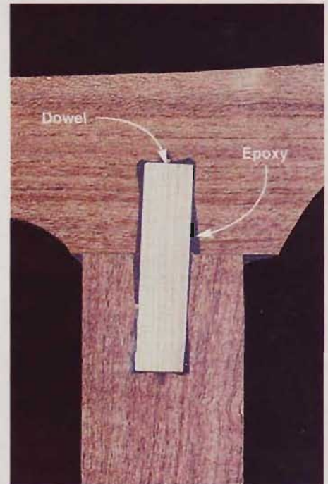
This arm/leg joint cutaway shows how the epoxy encapsulates the dowel in an over-size hole, strengthening the dowel.
