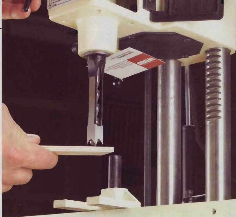
A business card between the chisel and mortiser head establishes the proper bit clearance during installation. The wood scrap protects your fingers from the chisel's sharp points.
