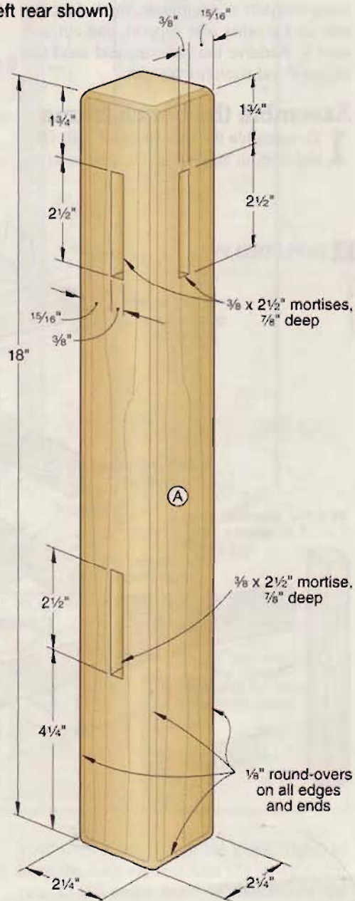
1 LEG (Left rear shown)
