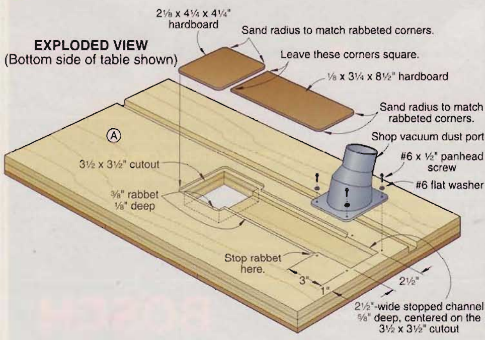
Rout a ⅜" rabbet ⅛" deep along the edges of the 3½"x3½" cutout and the edges of the 2½"-wide channel, stopping 3" from its end.
