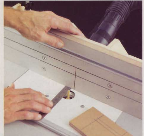
2 POSITION THE FENCE Chuck a slot-size bit in the router. Position the fence to center the bit in the slot.
