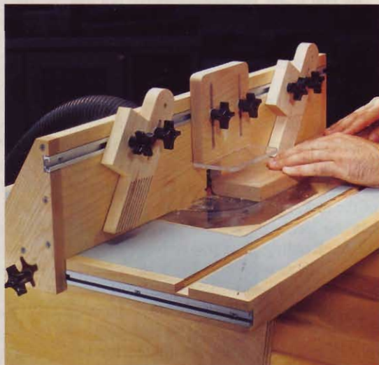
Our downloadable router-table plans allow you to build your own hard-working setup. The tilt-top model (left) offers storage, dust collection, and a large tabletop. The benchtop model boasts big features in a compact size.
