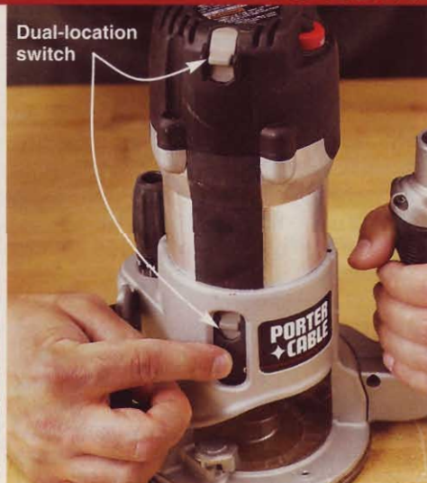
The Porter-Cable 895PK switch operates from two locations: at the base for handheld use, and at the motor top when table mounted.
