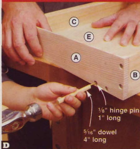
Using a 4"-long piece of \frac{5}{16} " dowel as a pin punch, drive the lid hinge pin flush with the bottom of the counterbore in the side (A).
