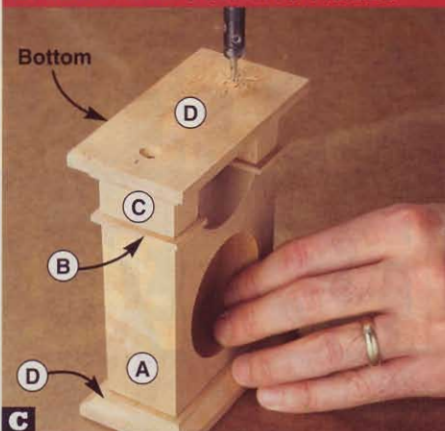
C Drill countersunk \frac{9}{64} " shank holes with \frac{3}{32} " pilot holes 1\frac{1}{4} " deep through the bottom (D), pillars (C), and plates (B) into the body (A).
