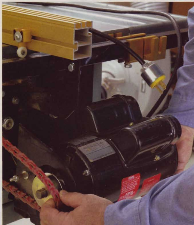
When installing a tablesaw tuneup kit, carefully align and tighten the machined pulleys. The flexible drive belt of interlocking segments keeps vibration to a minimum.
