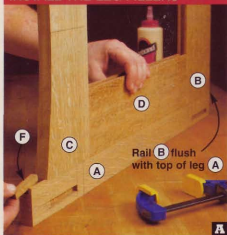
Dry-assemble a leg (A), top and bottom side rails (B, C), and center stile (D). With rail B flush with the top of the leg, glue and clamp a filler (F) in the leg groove tight to rail C.
