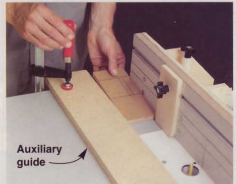
5 ADD AN AUXILIARY GUIDE Using the part width to gauge the distance, clamp an auxiliary guide parallel to the fence. Note: The part should slide easily between the guide and fence without excess play.
