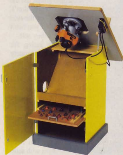
Our downloadable router-table plans allow you to build your own hard-working setup. The tilt-top model (left) offers storage, dust collection, and a large tabletop. The benchtop model boasts big features in a compact size.
