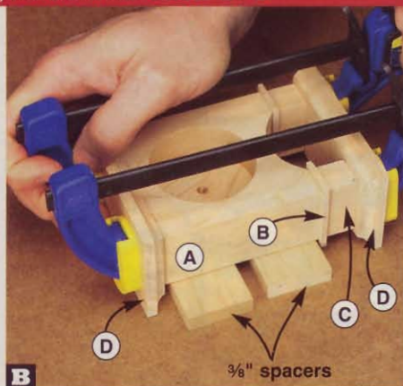
B With the body (A) on \frac{3}{8} " spacers, center the top and bottom (D) on the body side-to-side with a \frac{3}{8} " overhang, and clamp in place.
