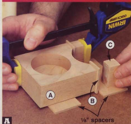
A Using \frac{1}{8} " spacers under the body (A) and pillars (C), center the pillars side-to-side on the plates (B), and clamp them in place.
