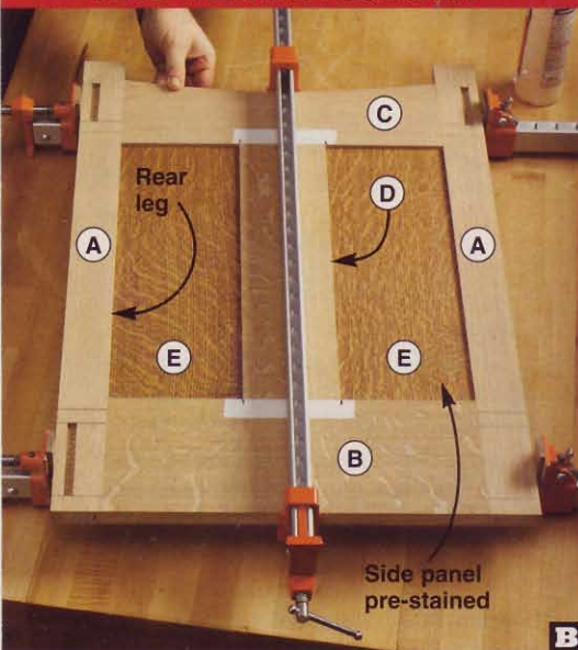
Assemble a side by gluing and clamping together two legs (A), top and bottom rails (B, C), center stile (D), and side panels (E), aligning the stile with the tape marks.
