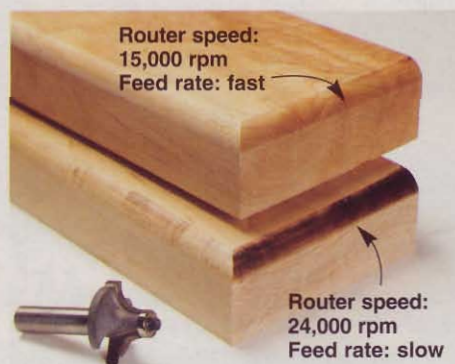
We used the same router and dull bit to round over these maple pieces (cut from the same board). The results are quite different.
