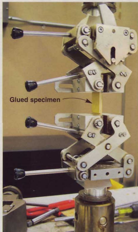
In Type 1 water-resistance testing, a glued specimen in wet and dry states is locked in jaws and subjected to shearing force.
