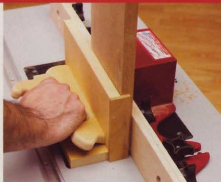
Carol's vertical pushstick, with a replaceable 1/4" plywood heel, helps you press tall pieces firmly against your router table fence.
