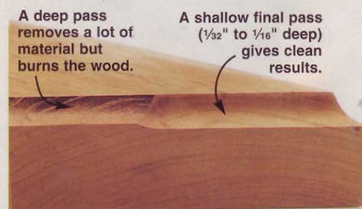
Even in burn-prone woods, such as cherry, making a shallow final pass keeps the bit and wood cool to eliminate most burns.
