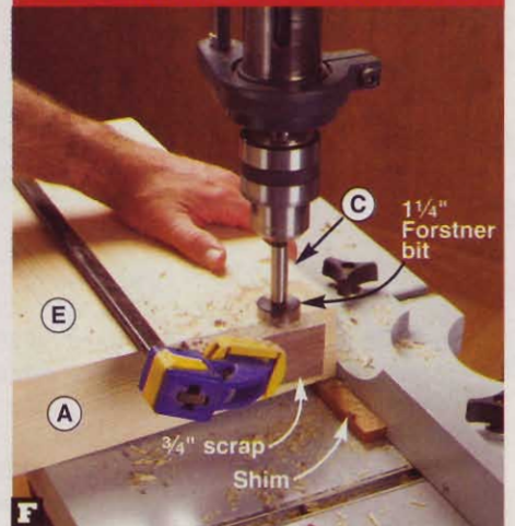
With the lap desk shimmed level and a \frac{3}{4} " scrap clamped to the side (A) to prevent tear-out, bore the turn-button recess.
