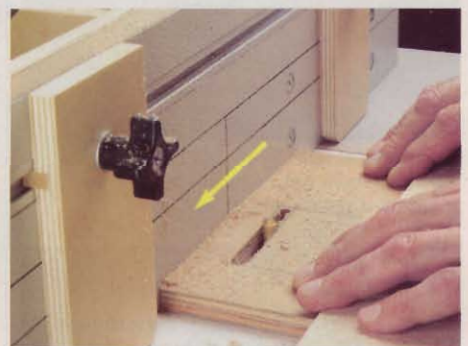
8 ROUT THE SLOT Feed the part to the left until it hits the stop. The auxiliary guide keeps the part in line.
