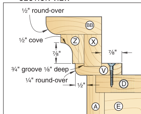
7a CROWN MOLDING SECTION VIEW
