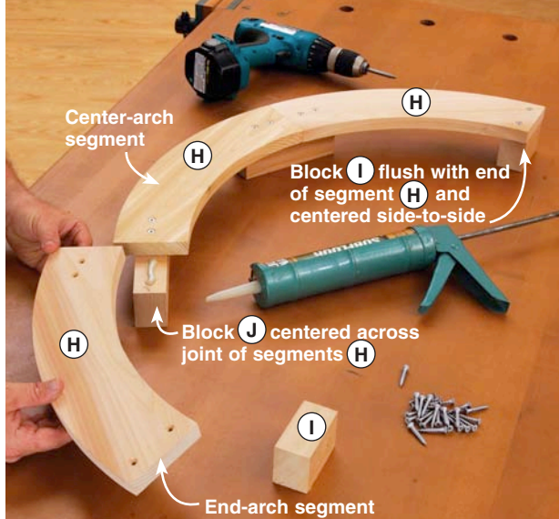
B FORM THE SEGMENTED ARCH Fasten two end-arch segments (H) and a center-arch segment to the mounting blocks (I, J), positioning the blocks as shown.
