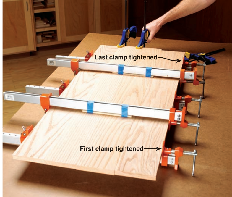
MOVE JOINT CLAMPS TO THE OPPOSITE END
