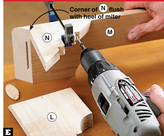
E Using the screw holes in the corner blocks (N) as guides, drill pilot holes into the base front (M), and drive the screws.
