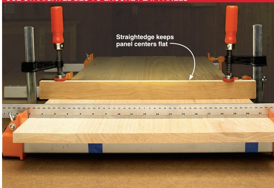
USE STRAIGHTEDGES TO ENSURE FLAT PANELS
