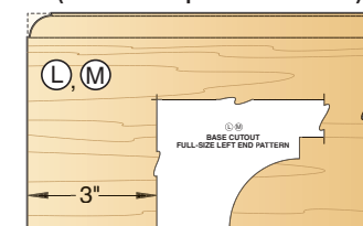
5a PATTERN LOCATION (Left-hand pattern shown)
