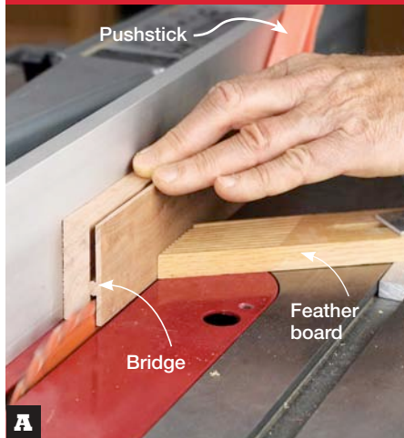
A Between the kerfs, leave a bridge about \frac{1}{2} " wide. The bridge can be removed later with a bandsaw or handsaw.
