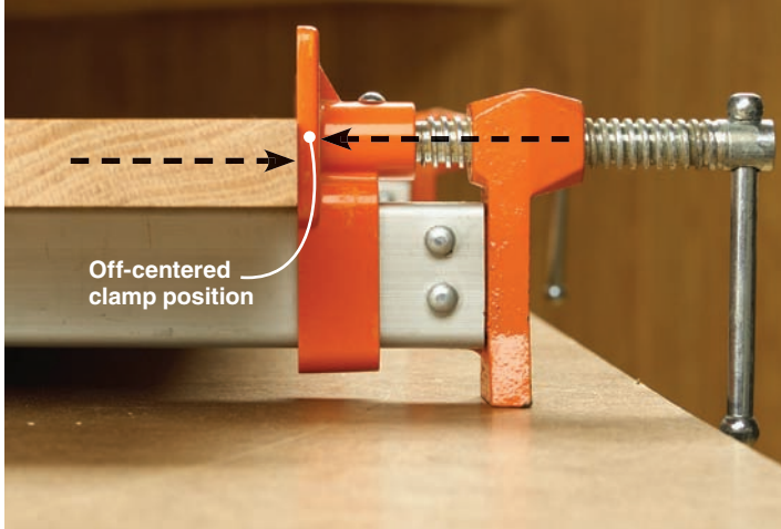
THE PROBLEM: MISALIGNED CLAMP PRESSURE
