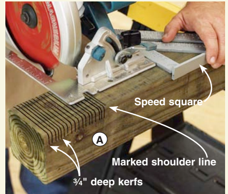
Step 1: Using a guide, such as a speed square, cut a series of kerfs approximately 1/8" apart across the width of the marked rabbet, stopping at the shoulder line.
