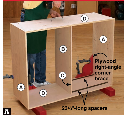
A Align the divider (B) with spacers. Using the holes in the case top and bottom (D) as guides, drill pilot holes and drive the screws.
