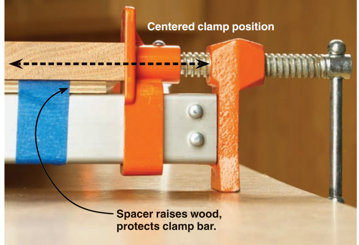
THE SOLUTION: CENTER CLAMPING PRESSURE
