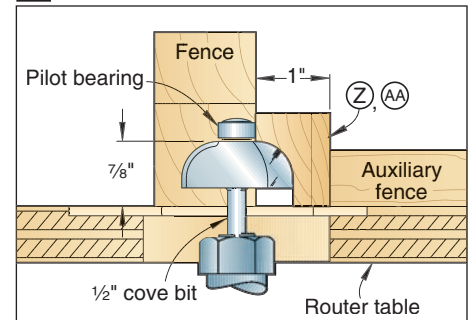
7b FORMING THE COVES
