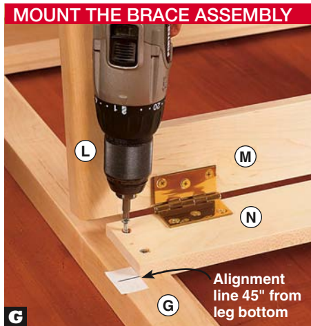
G Holding the brace assembly up, align the bottom edge of the hinge rail (N) with the marked lines. Drill pilot holes, and drive the screws.
