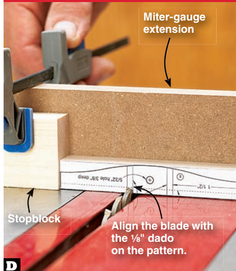
D Align the blade with the 1/8" dado shown on the gripper (E) pattern. Clamp a stopblock to the miter-gauge extension.
