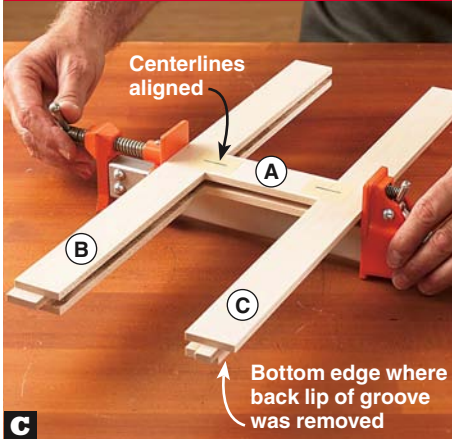
C Aligning the marked centerlines, glue and clamp the center stile (A) between the top rail (B) and center rail (C). Centerlines aligned Bottom edge where back lip of groove was removed
