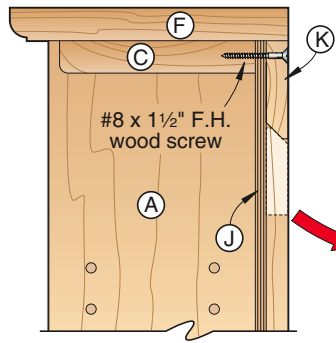
4 CASE SECTION VIEW (Left case shown)
