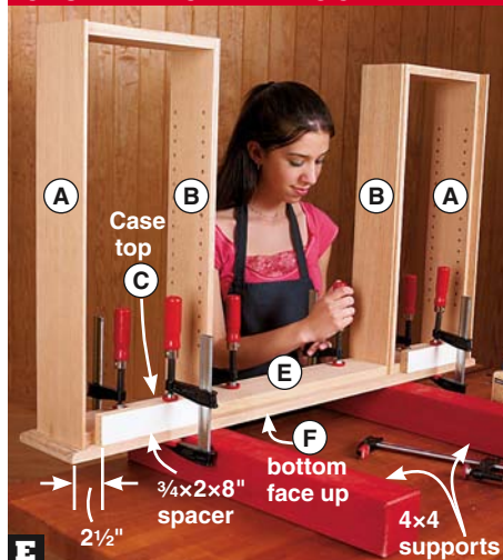
Glue and clamp the cases and a case spacer (E) to the top (F), keeping the case tops (C) tight against \frac{3}{4} " spacers clamped to the top.
