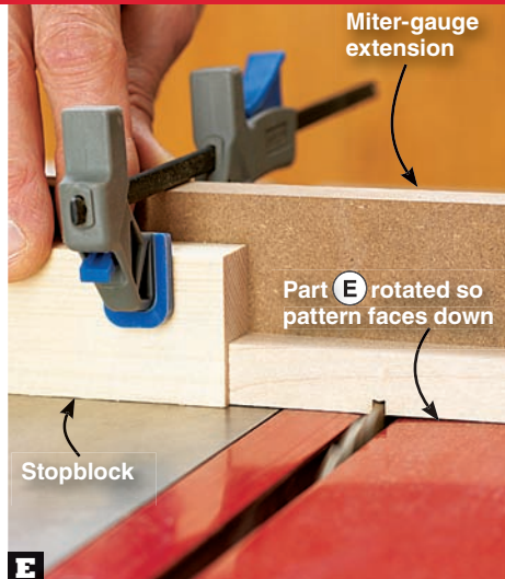
E Rotate the gripper (E) blank so the pattern faces down and cut the dado. Then turn the blank end-for-end and dado the other end.
