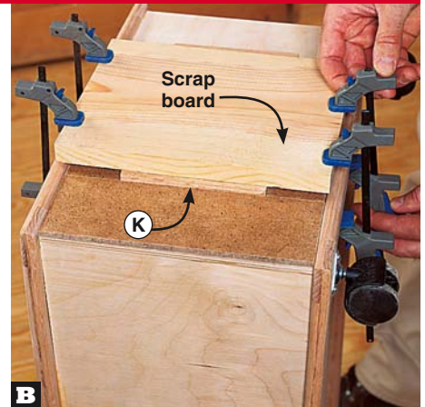
B Place a scrap board on the cleats (K, L) and apply pressure with clamps. Remove the side cleat/panel assembly (K/M).
