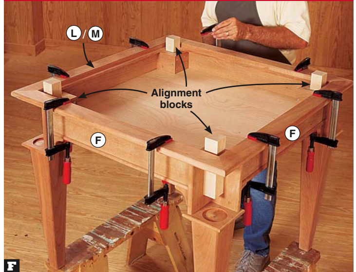
F Apply a thin bead of glue to the top edges of the aprons (F). Lower the top frame (L/M) over the alignment blocks, and clamp it in place.
