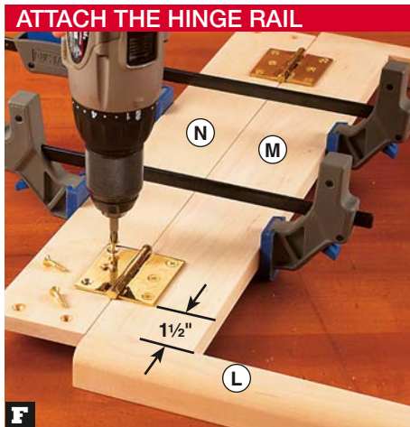
F Position 2½x2" brass butt hinges on the top rail (M) and hinge rail (N), where shown. Drill pilot holes, and drive the screws.
