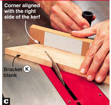
C Turn the bracket stock over. Align the corner with the right side of the saw kerf, and cut off a bracket blank. Repeat to make four blanks.
