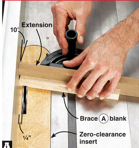
Angle the miter gauge 10° to the right and attach an extension. With the brace (A) blank corner touching the fence, cut the first dado.
