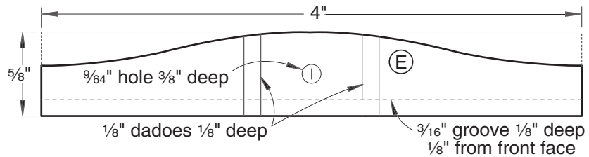
FULL-SIZE FOOT PATTERN (Back face)
