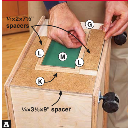
A Apply glue to one side cleat (K) and top and bottom cleats (L) and use spacers and the panel (M) to position them on the front (G).
