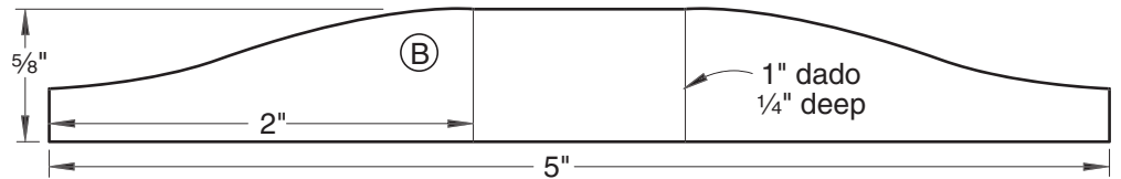
FULL-SIZE FOOT PATTERN (Back face)
