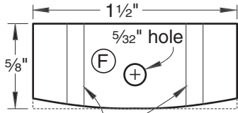
FULL-SIZE CLAMP PATTERNS (Front view)
