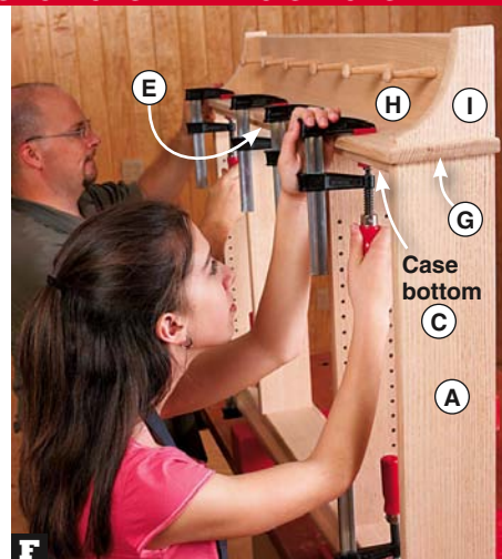
Then glue and clamp the peg-rail assembly (G/H/I) and remaining case spacer (E) in place, aligning them as shown.
