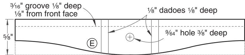
FULL-SIZE GRIPPER PATTERNS (Back faces)
