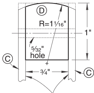
FULL-SIZE CAP PATTERN
