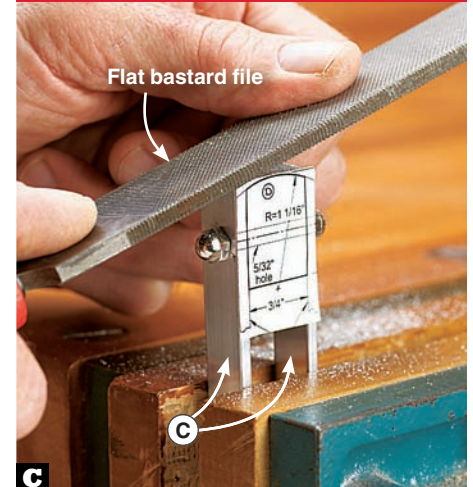
Rough-form the curved top of the uprights (C) and cap (D) with a flat bastard file. Then finish-sand with sandpaper to 220 grit.
