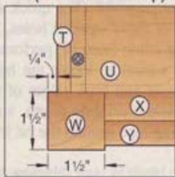
5a PILLAR LOCATION DETAIL (Viewed from top)
