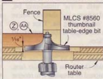
5b TRIM THUMBNAIL DETAIL
