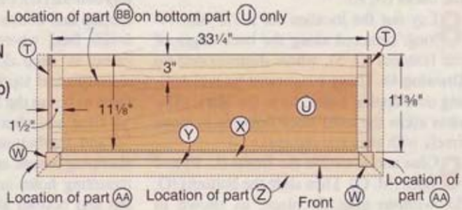
5c TRIM LOCATION DETAIL (Viewed from top)
