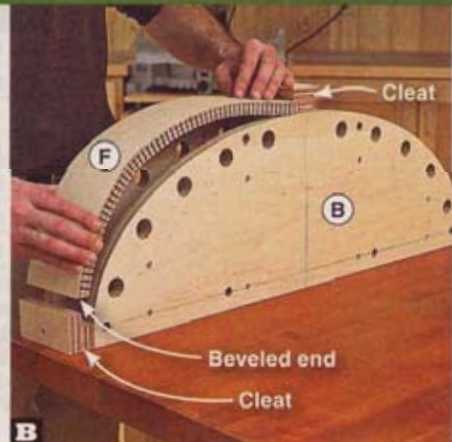
B Orienting the beveled end of the apron (F) as shown, tuck the ends under the overhanging edges of the cleats.
