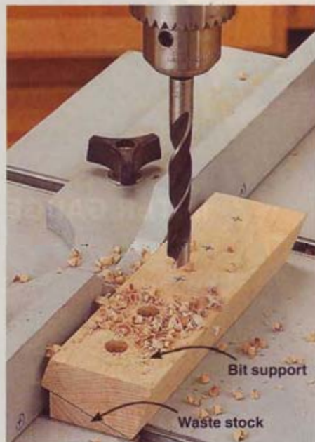
Stick the waste stock to the bit support, and drill the 1/2" holes.
