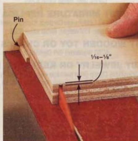
Place one end of the workpiece against the pin, and cut the first saw kerf.
