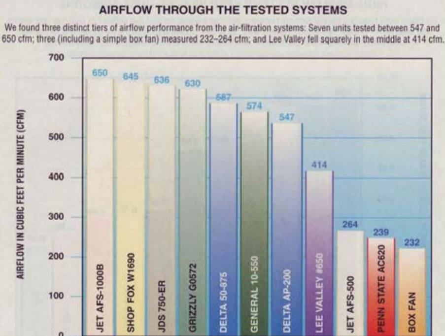
Airflow measured with hot-wire anemometer at 25 distinct points 1¼' from the prefilter face. To test real-world airflow, filters were loaded under identical circumstances, and then tapped clean before airflow measurements were taken. Numbers shown are an average of three tests.
