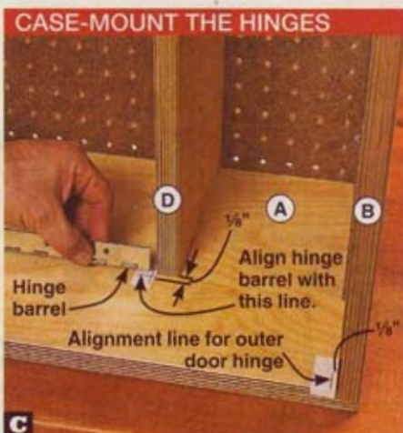
C Align the inner-door hinge with the marked lines, and press the taped hinge in place. Then drill the mounting holes.
