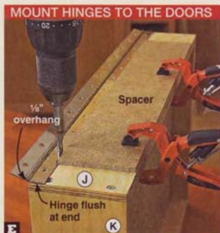
E Clamp the spacer to the door, flush with the back edge. With the hinge tight against the spacer, drill the mounting holes.
