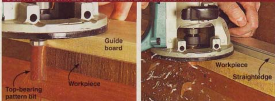
Rest your router subbase on top of the guide board and run the bearing against its edge. Trim no more than \frac{1}{16} " per pass.
