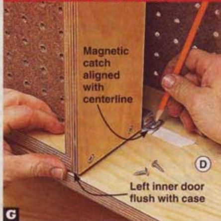
G Align the mounting flange of the magnetic catch with the marked centerline on the shelf (D). Mark the centers of the slots.
