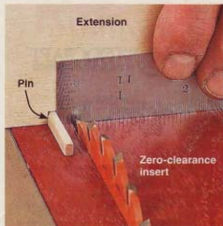
Position the pin \frac{1}{4} " from the blade, and fasten the extension to the miter gauge.
