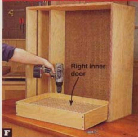
F Position the right inner door in the case, aligning the hinge with the previously drilled mounting holes. Drive the screws.
