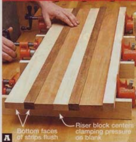
A Glue and clamp the contrasting wood strips together in order, keeping the bottom faces and ends flush.
