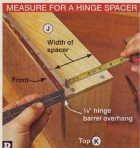
D Position a hinge on an inner-door side (J) with a \frac{1}{8} " overhang. Measure from the back to the hinge to find the spacer width.
