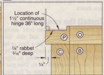
5c BACK CAP TRIM SECTION DETAIL
