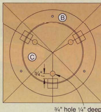
\frac{3}{4} " hole \frac{1}{4} " deep
