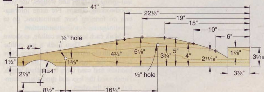
3 BENDING FORM SIDE VIEW
