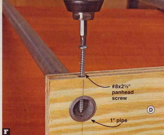
F SCREW-MOUNT THE OUTER RESTS
