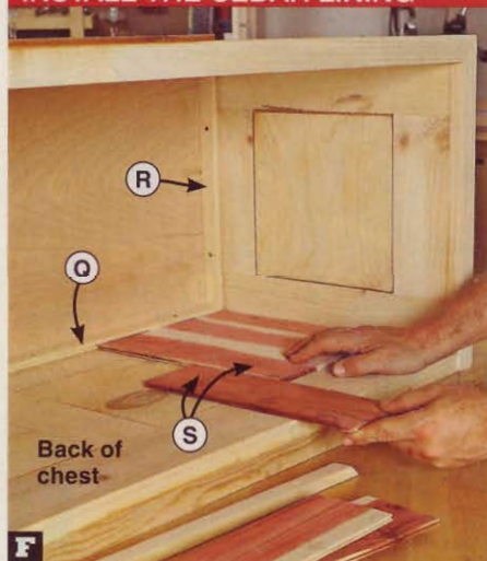
F Slide each piece of the back lining (S) into the rabbet in the bottom back lining retainer (Q), keeping the lining joints tight.
