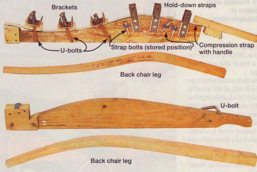
The top form makes compound curves using a mix of screw-down brackets and straps plus a compression strap. The right end of the form holds the compression strap handle in place. The lower form creates a simple curve, using two U-bolts and wedges. The maple and walnut slat form at right is modeled after one used in the middle to late 1700s.
