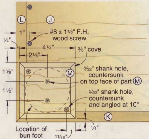
5a FOOT SUPPORT MOUNTING DETAIL (Viewed from bottom)
