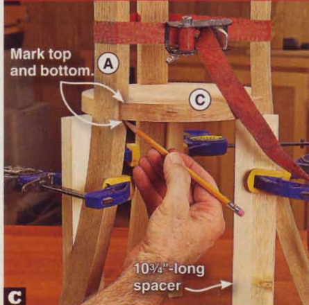
C Clamp the legs (A) into the shelf (C) notches, positioning the shelf with 10 3/4"-long spacers. Mark the shelf top and bottom on one leg.
