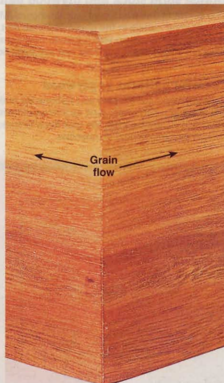
Cutting four box pieces from a single board lets the grain flow around the corners.
