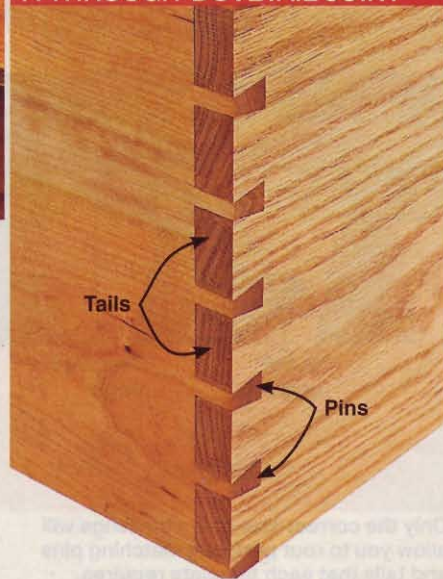
A THROUGH-DOVETAIL JOINT
