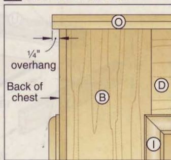
5b END VIEW DETAIL
