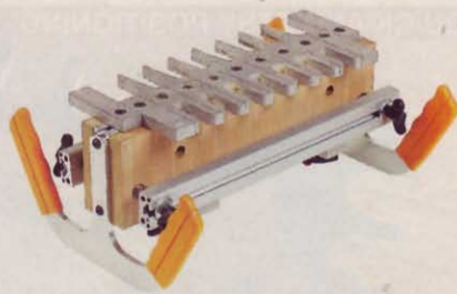
Katie Jig KJ12000002, $260, fully equipped for through dovetails 317/881-8601; katiejig.com
