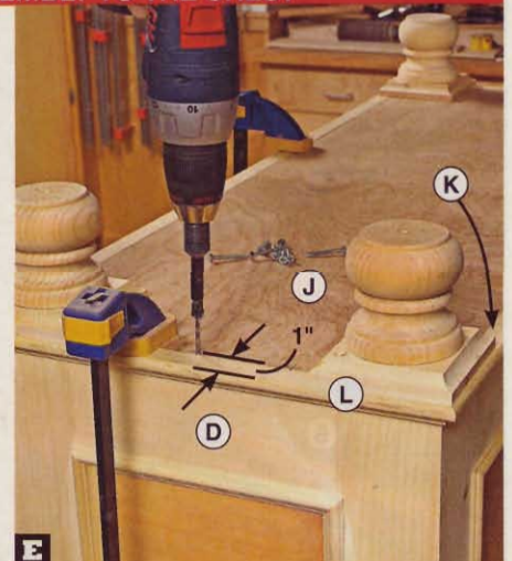
E Drill mounting holes 1" from the outside edges of the front/back and side trim (K, L) to mount the bottom assembly to the chest.
