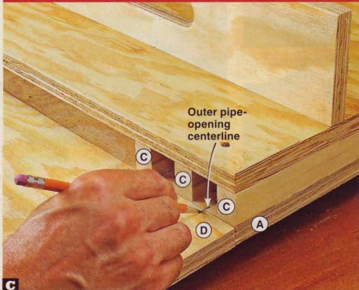
C With the ends of an extension rest (D) aligned with the bottom platform (A), extend the centerlines from the pipe openings.
