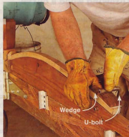
If bent quickly after being pulled from the steam chamber, this workpiece will easily wrap across the form.
