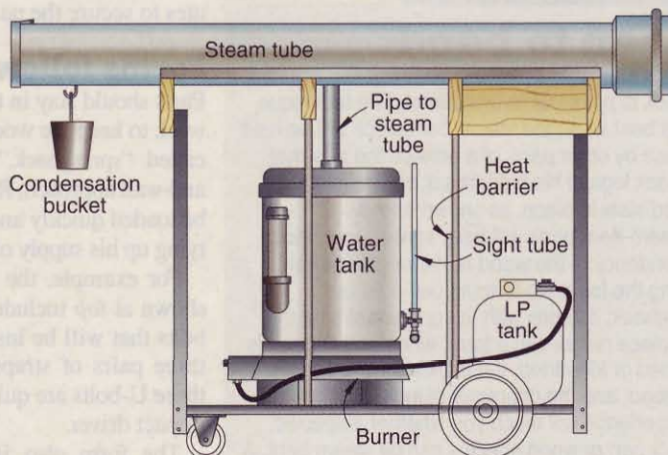
Russ's steamer uses a 22-quart water tank from a recycled steel pressure cooker to avoid refills while steaming.
