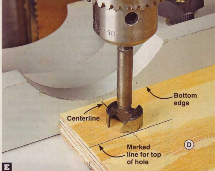
E BORE THE EXTENSION RESTS
