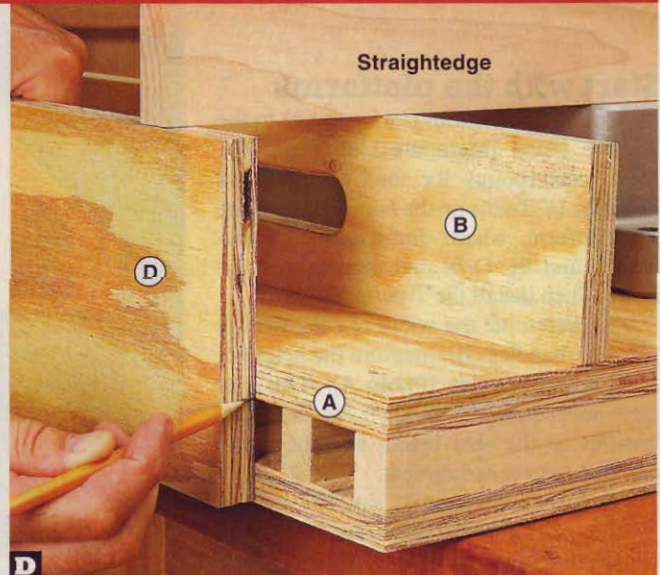
D Flip the rest up 90°. Then mark the location of the bottom of the top platform (A) on the end of the rest.
