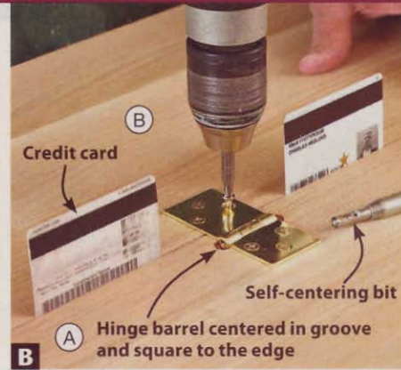
B Insert credit cards 1 / 8 " into the rule joint to separate the top (A) and leaf (B), drill pilot holes, and install the hinges.
