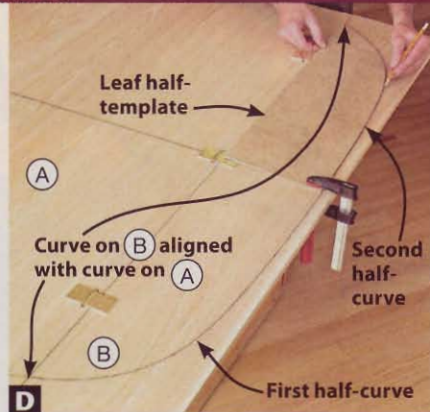
Align the template with the top (A) end curve, and draw half the leaf (B) curve. Flip the template, and complete the curve.
