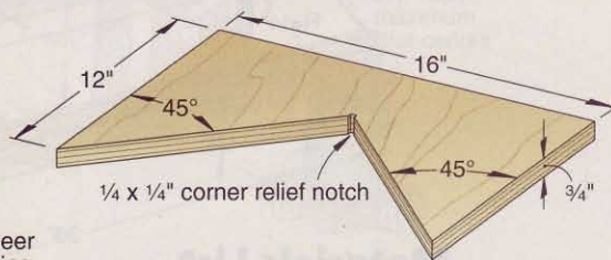
7 TRIANGLE-CUTTING JIG
