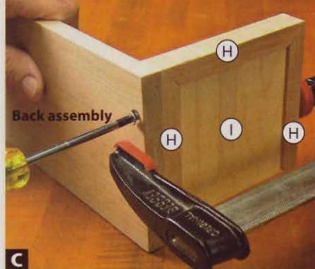
C SCREW-MOUNT THE TRAYS With the trays (H/I) glued and clamped to the back assemblies, drive the screws through the holes in the backs into the trays.
