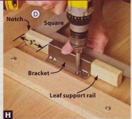
H Center the leaf support rail in the side skirt (D) notch, and square the support bracket to the skirt. Drill pilot holes, and drive the screws.
