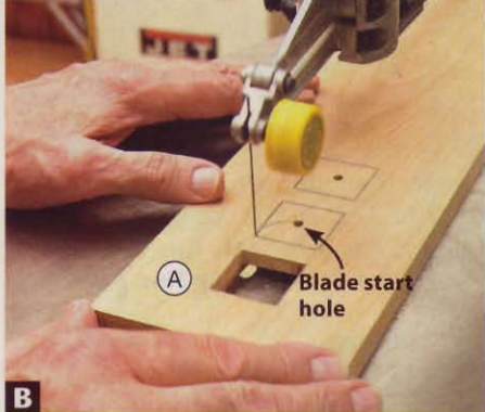
B SCROLLSAW THE BACK OPENINGS Insert your scrollsaw blade through the blade start hole, and cut out each of the 1 1/4"-square openings in the backs (A, B, C).
