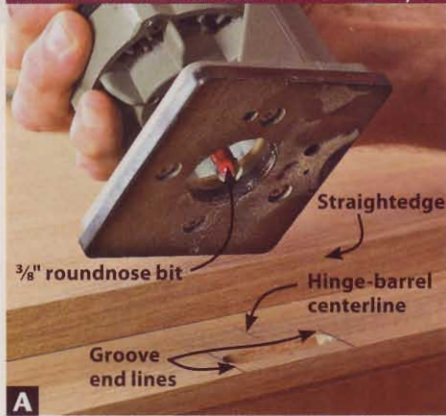
A Position a straightedge to center a 3 / 8 " roundnose bit on the hinge-barrel centerline, and rout a 3 / 16 "-deep groove for each hinge.
