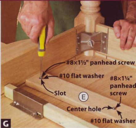
G After using the stretcher (E) center hole and slot centers as guides to drill pilot holes, fasten them with washers and screws.
