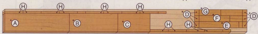
¾ x 5½ x 60" Cherry (2.5 bd. ft.) *Plane or resaw to the thicknesses listed in the Materials List.
