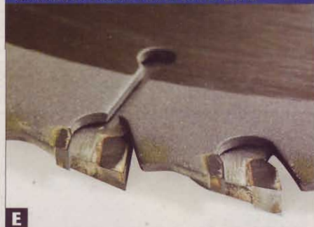
E Blades with large carbide teeth, like the Forrest Woodworker II (bottom), can be sharpened more times than those with small teeth, like the Irwin Marathon (top).
