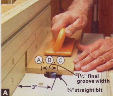
A ROUT GROOVES INTO THE BACKS Widen the centered 1/4"-deep groove in the backs (A, B, C) by making two passes, rotating the parts 180° between the passes.
