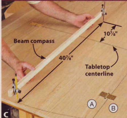
Lay out the centers of the top (A) end radii from the tabletop centerline, and use a beam compass to draw the curves.
