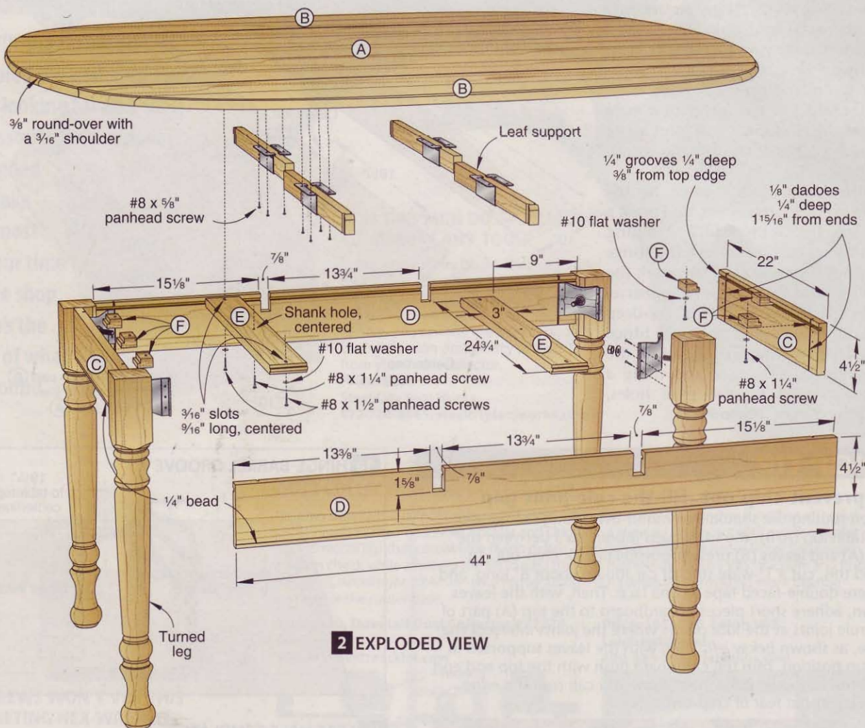
Lay out the centers of the top (A) end radii from the tabletop centerline, and use a beam compass to draw the curves.
