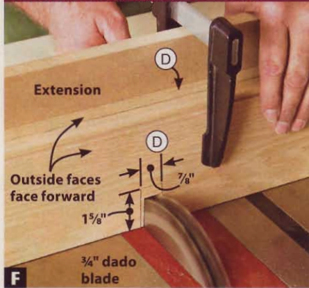
F Using a tall miter-gauge extension to support the side skirts (D) and back the cuts, cut the leaf-support notches in two passes.
