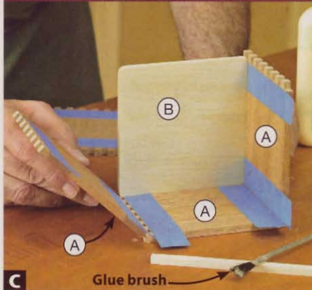
C Protect the inside faces of the sides (A) with masking tape. Then brush glue onto the fingers, and assemble the box.
