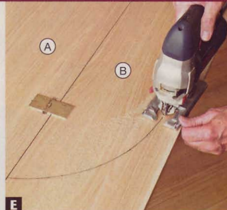
With the top (A) end curves and the leaf (B) side curves drawn, cut the tabletop to shape with a jigsaw.
