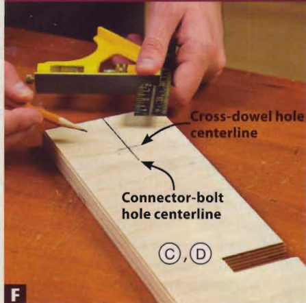
F Using a combination square, mark the centerline of the \frac{3}{32} " connector-bolt hole and the center of the 10mm cross-dowel hole.
