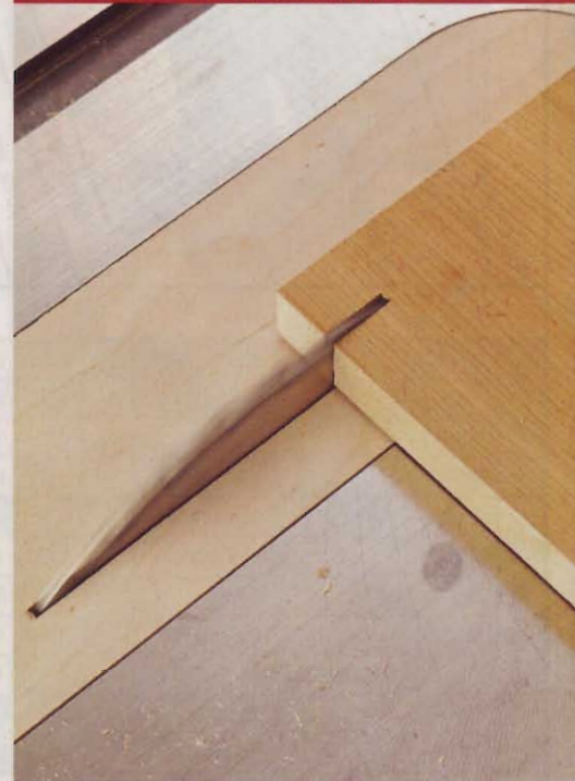
This shop-made zero-clearance insert fully supports delicate veneer fibers as the blade's teeth exit the cut.
