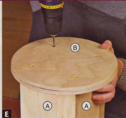
E With the foot (B) seated on the leg side (A) assembly, use the holes in the foot as guides, and drill pilot holes into the leg sides.
