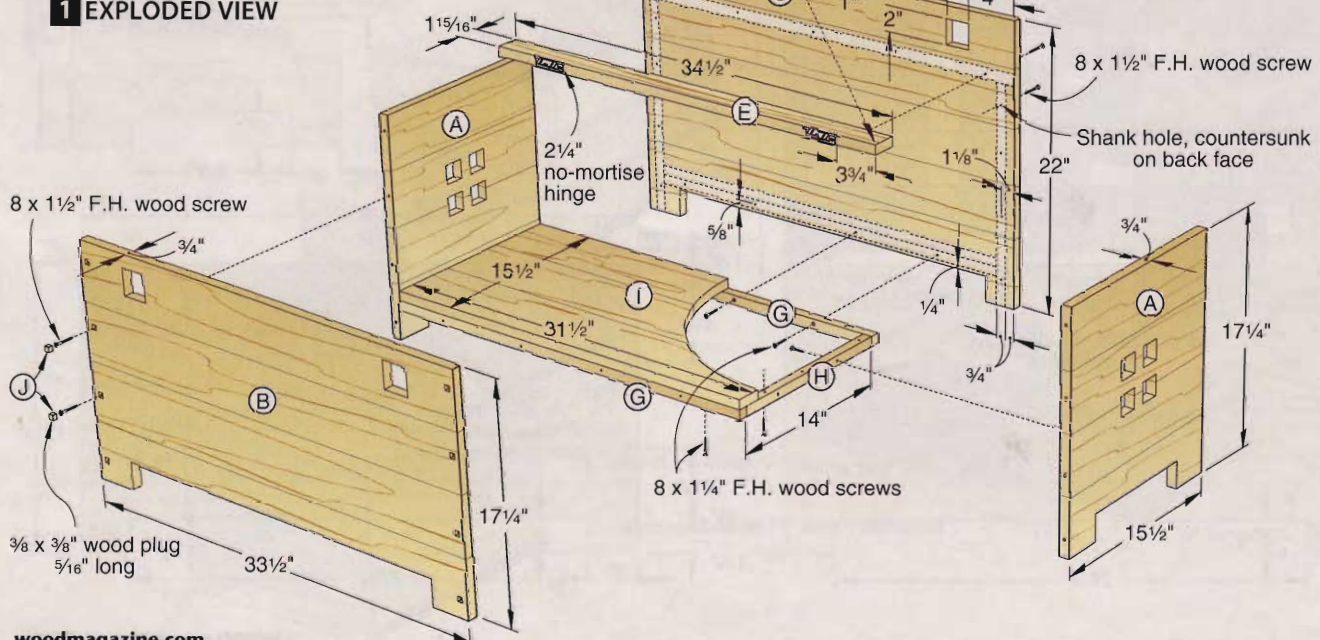
With the marked square openings in the sides (A), front (B), and back (C) overhanging your workbench, jigsaw out the openings.
