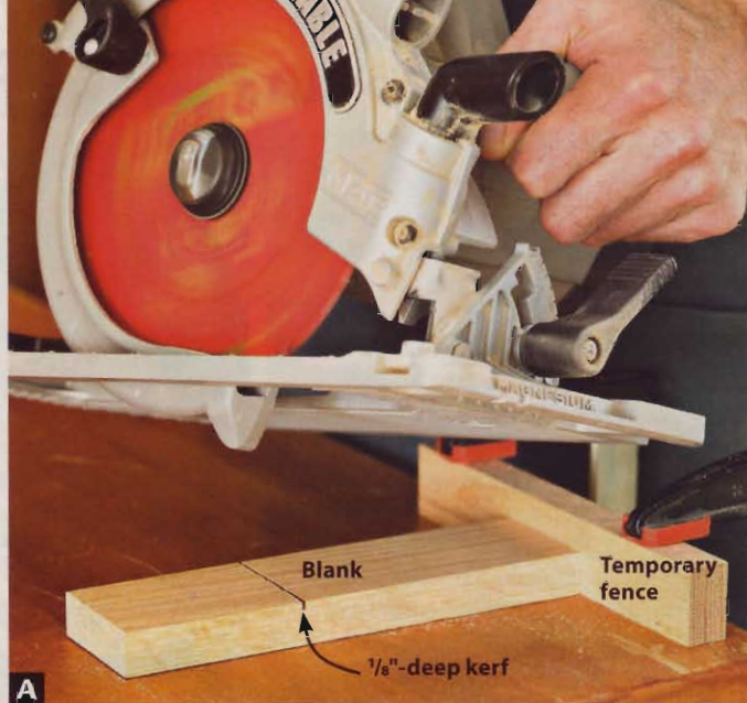
A Clamp the blank and temporary fence to the workbench. Holding the circular saw base against the fence, cut a \frac{1}{8} "-deep kerf.
