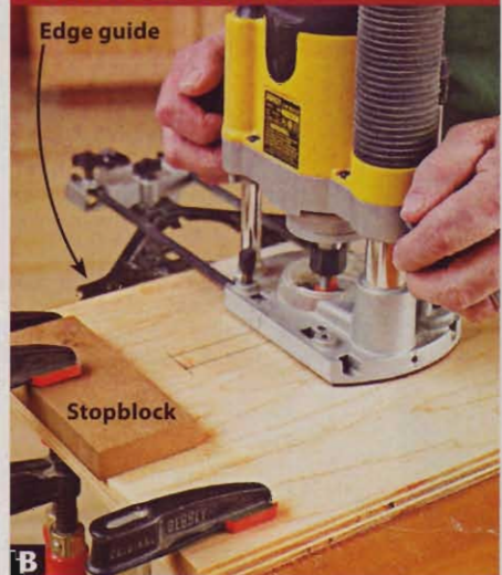
B When using a plunge router with stopblocks, be sure your clamps do not impede the router or edge guide.
