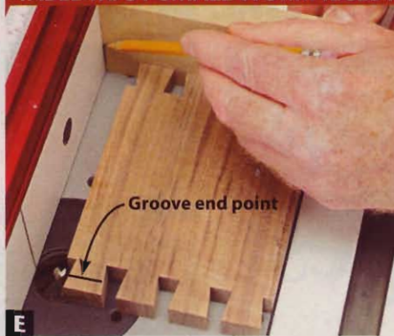
E Set the endpoint at the bit's left cutter edge, and mark a stopping point on the fence at the other end. Repeat for the opposite end.
