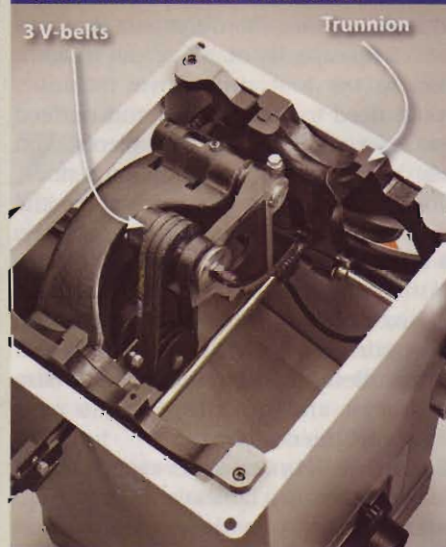
The trunnions on this Steel City saw, as well as on Craftsman's hybrid, mount to the cabinet rather than the top.
