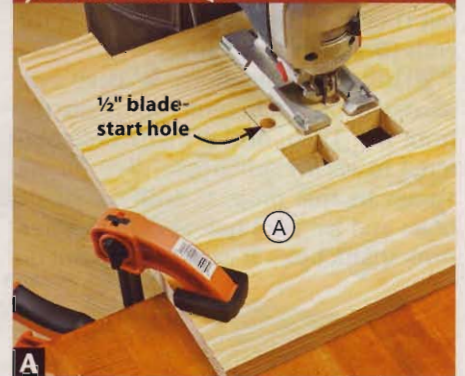
With the marked square openings in the sides (A), front (B), and back (C) overhanging your workbench, jigsaw out the openings.
