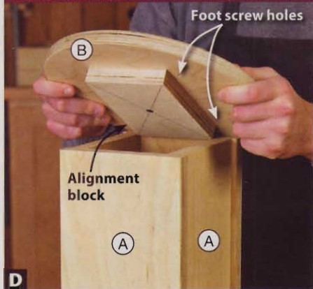
D With a block screwed to a foot (B), and aligned with the foot screw holes, position the foot on a leg side (A) assembly.
