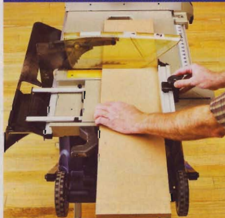
Ryobi's job-site saw features a sliding crosscut table that locks into place when you want to make a rip cut or for storage.
