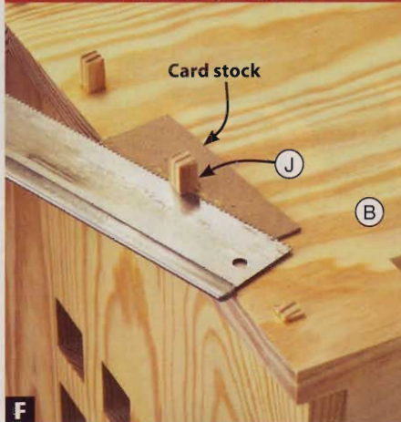
F Place a piece of approximately \frac{1}{16} "-thick card stock with a hole in it over each plug blank. Trim the plugs using a fine-tooth saw.
