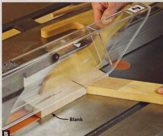
B Remove the temporary fence from the blank and rip the blank in half to make two 1"-wide setup gauges.
