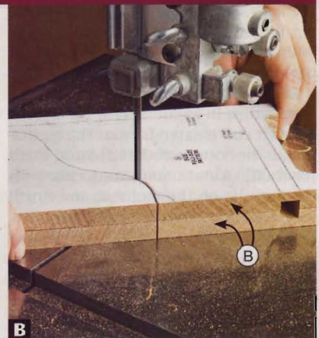
B With the bottom cutouts finish-sanded, separate the sides (B) from the back (A), and stack-cut the upper profile in both sides.
