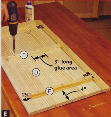
E Glue and screw the top cleats (F) to the top (D). Apply glue to only a center 3"-long area on the cleat to allow for top movement.
