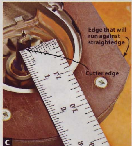
C The distance between the edge of the router base and the bit's cutter ( 2\frac{9}{16} " in this case) tells you where to position the stopblock.
