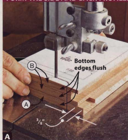
A Adhere the sides (B) to each other and the back (A) with double-faced tape and stack-cut the bottom cutouts.
