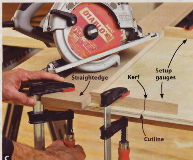
C With the setup gauges clamped to the panel, position the straightedge against the ends of the gauges, and clamp it in place.
