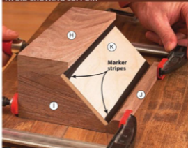
C Draw black marker stripes about \frac{1}{8} " wide on the front of the support (K) to keep the plywood from showing behind the ring bar.
