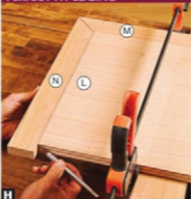
Clamp two mitered edging pieces (M, N) to a top panel (L), and mark their final lengths. Keep all faces flush as you glue them in place.
